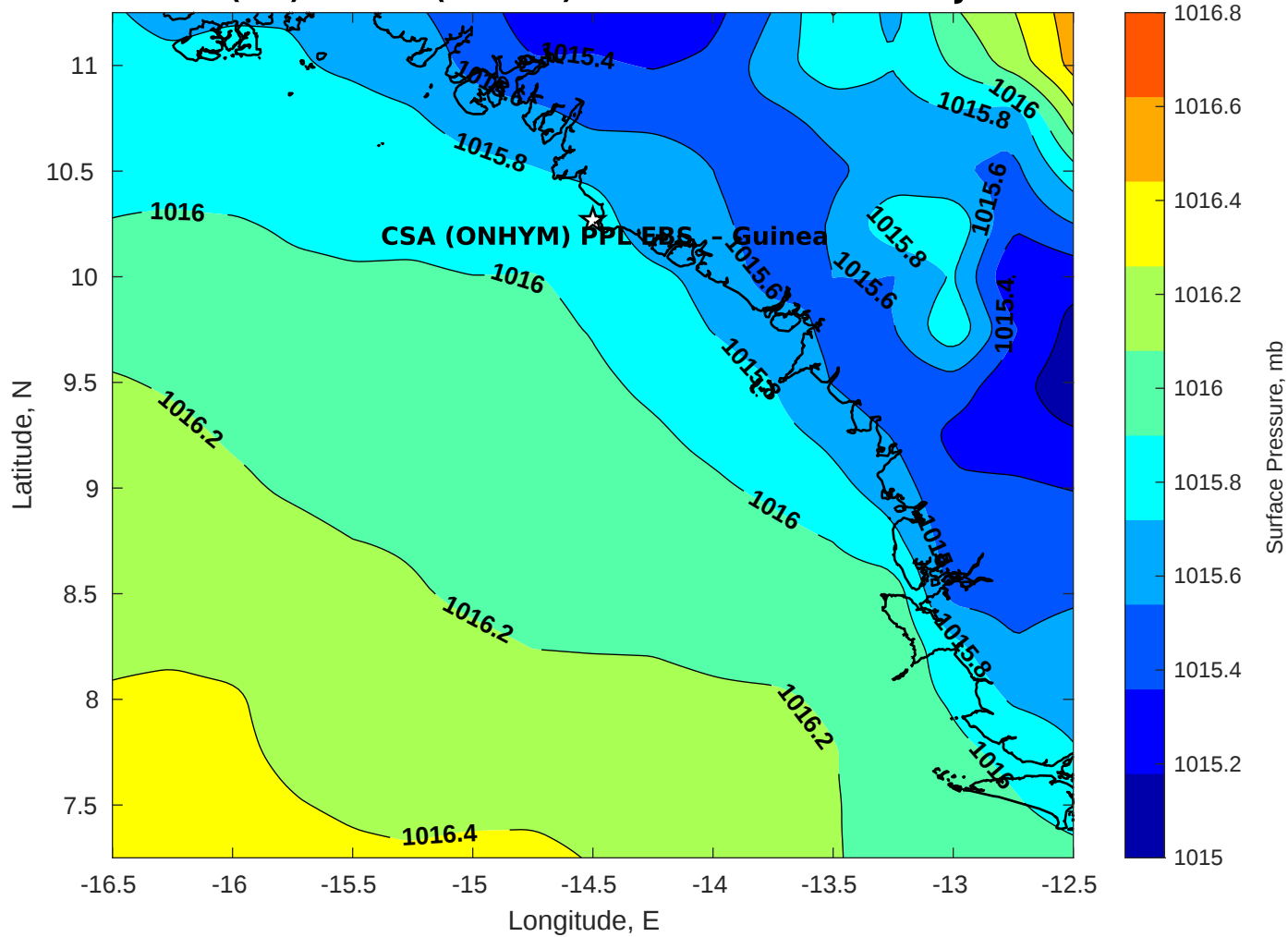
Surface Pressure (mb) for CSA (ONHYM) PPL EBS - Guinea at 20-Jul-2025 12:00:00
