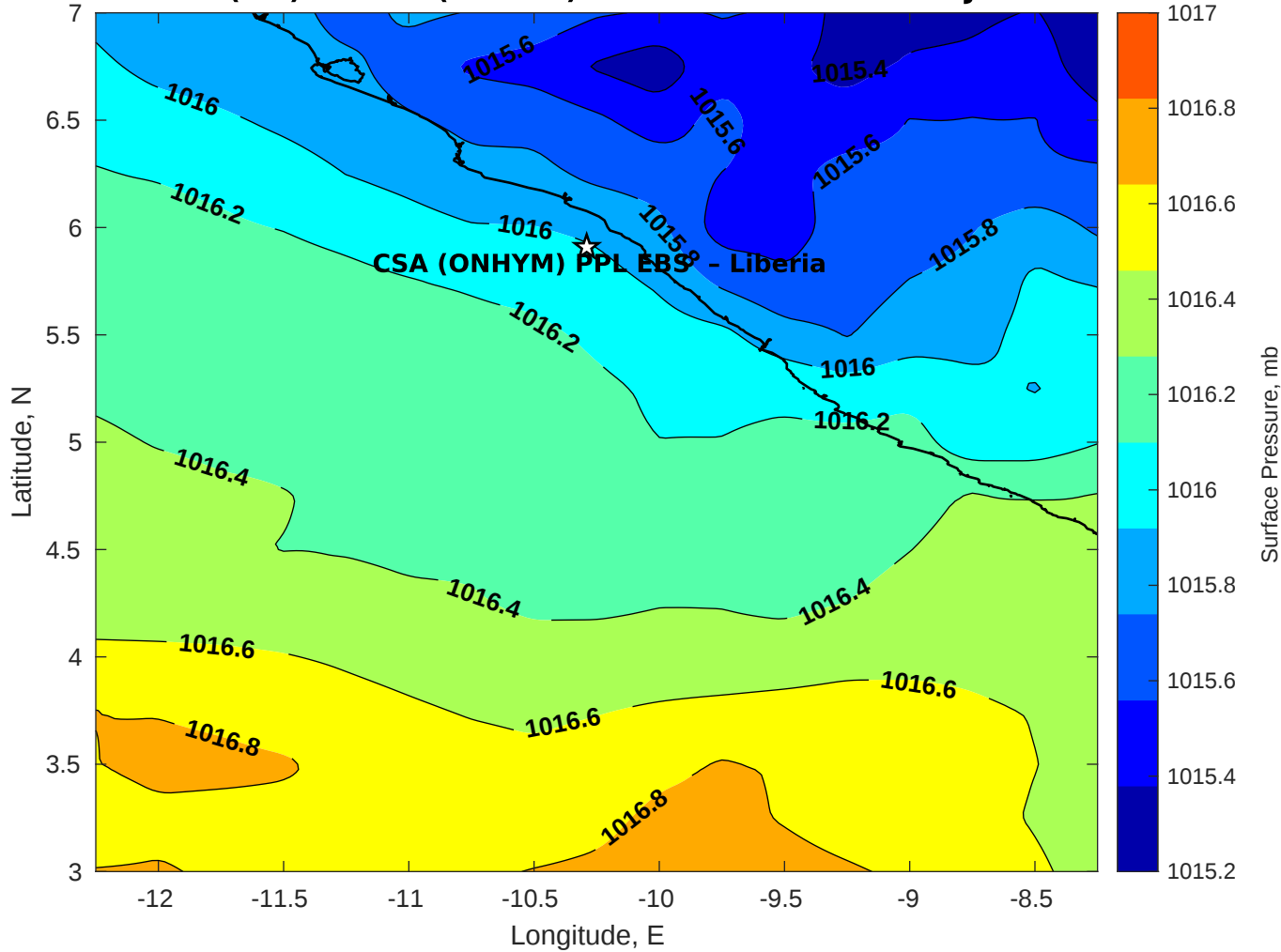
Surface Pressure (mb) for CSA (ONHYM) PPL EBS - Liberia at 20-Jul-2025 12:00:00
