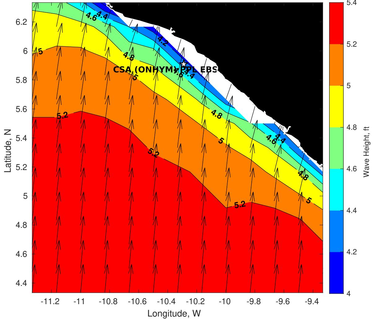
Wave Height (ft) for CSA (ONHYM) PPL EBS - Liberia at 19-Jul-2025 21:00:00
