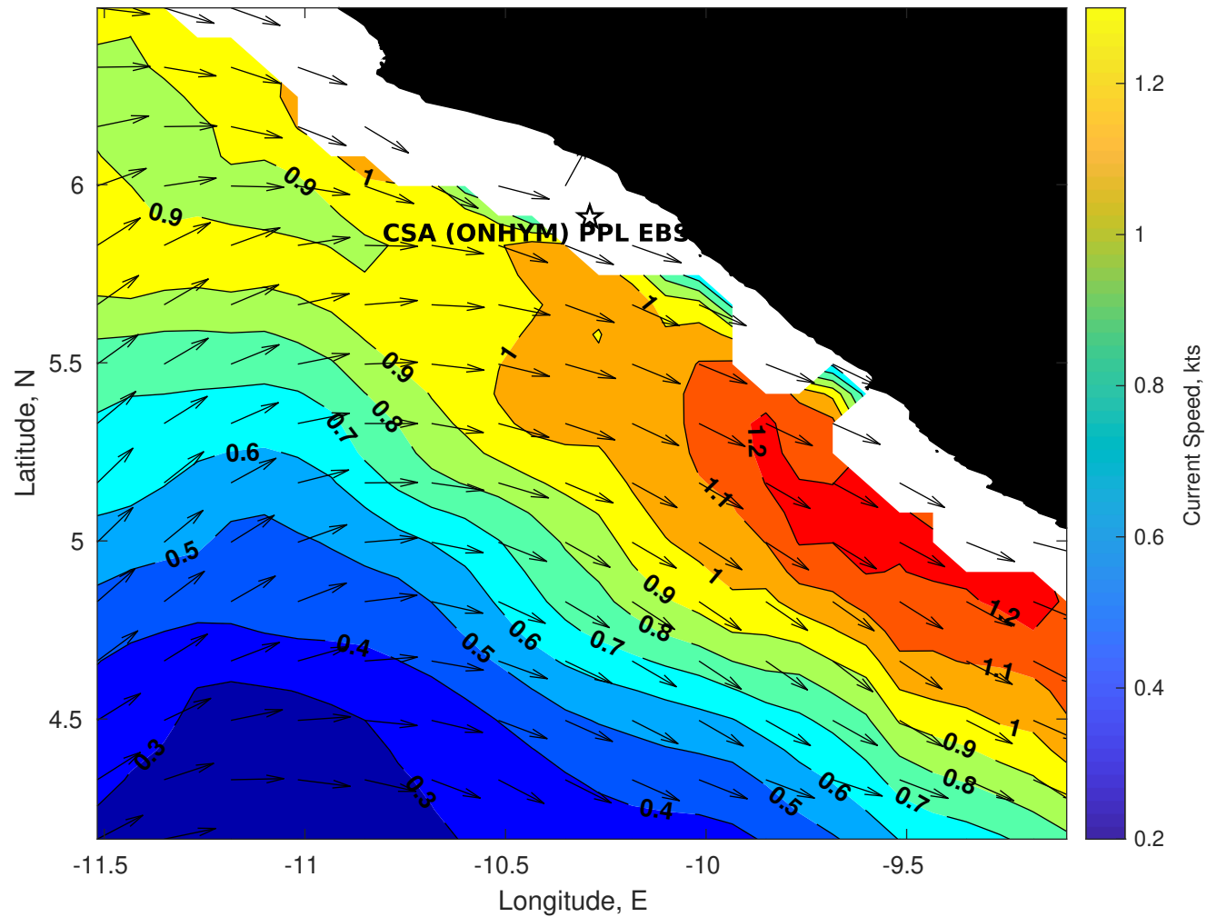
Surface Currents for CSA (ONHYM) PPL EBS - Liberia at 19-Jul-2025 00:00:00
