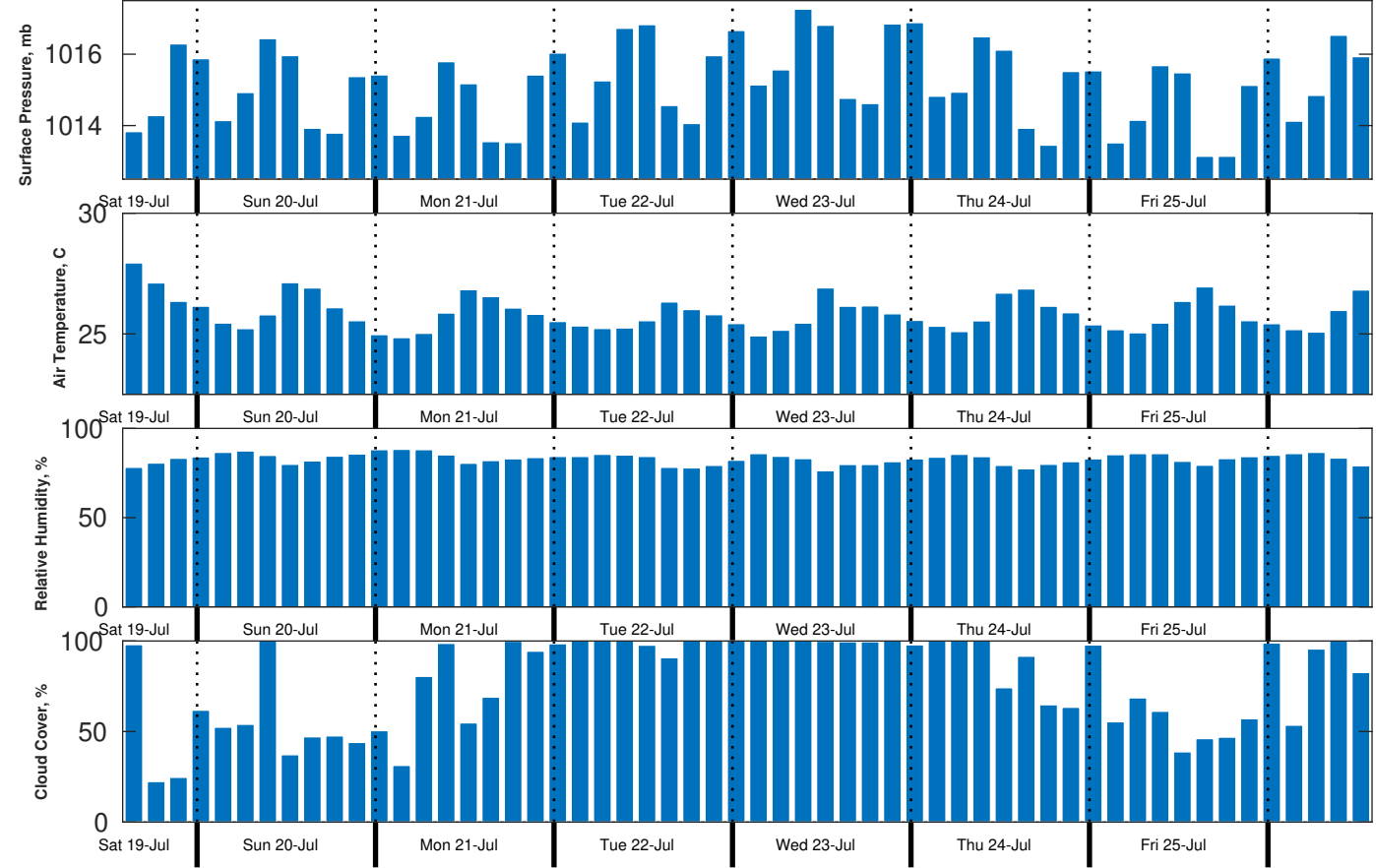
Met Forecast for CSA (ONHYM) PPL EBS - Liberia from 19-Jul-2025 12:00:00 to 26-Jul-2025 12:00:00
