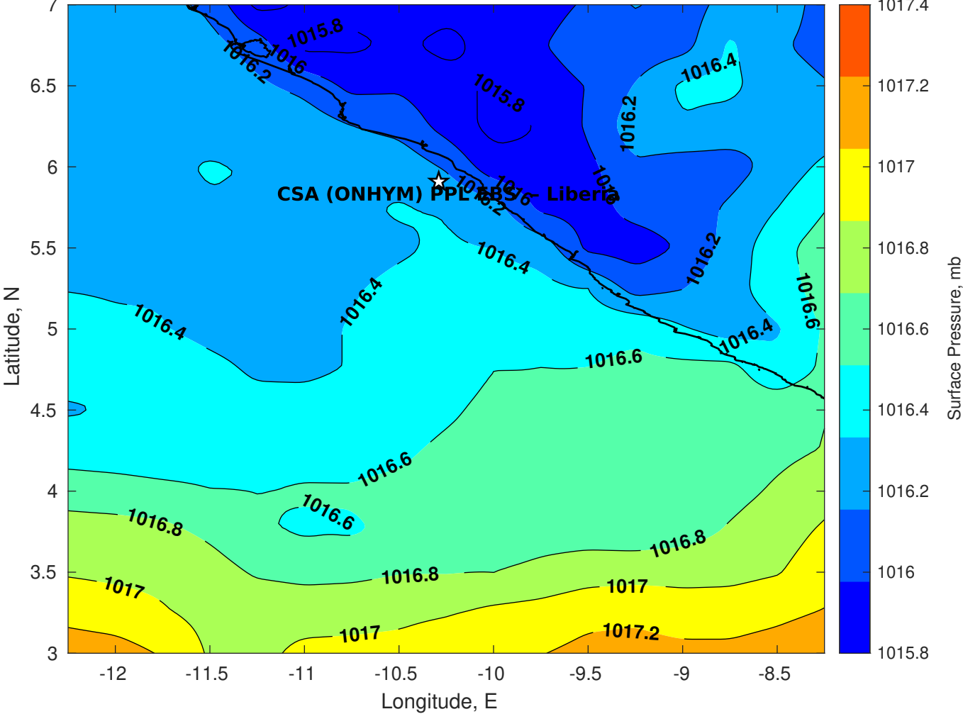
Surface Pressure (mb) for CSA (ONHYM) PPL EBS - Liberia at 19-Jul-2025 12:00:00
