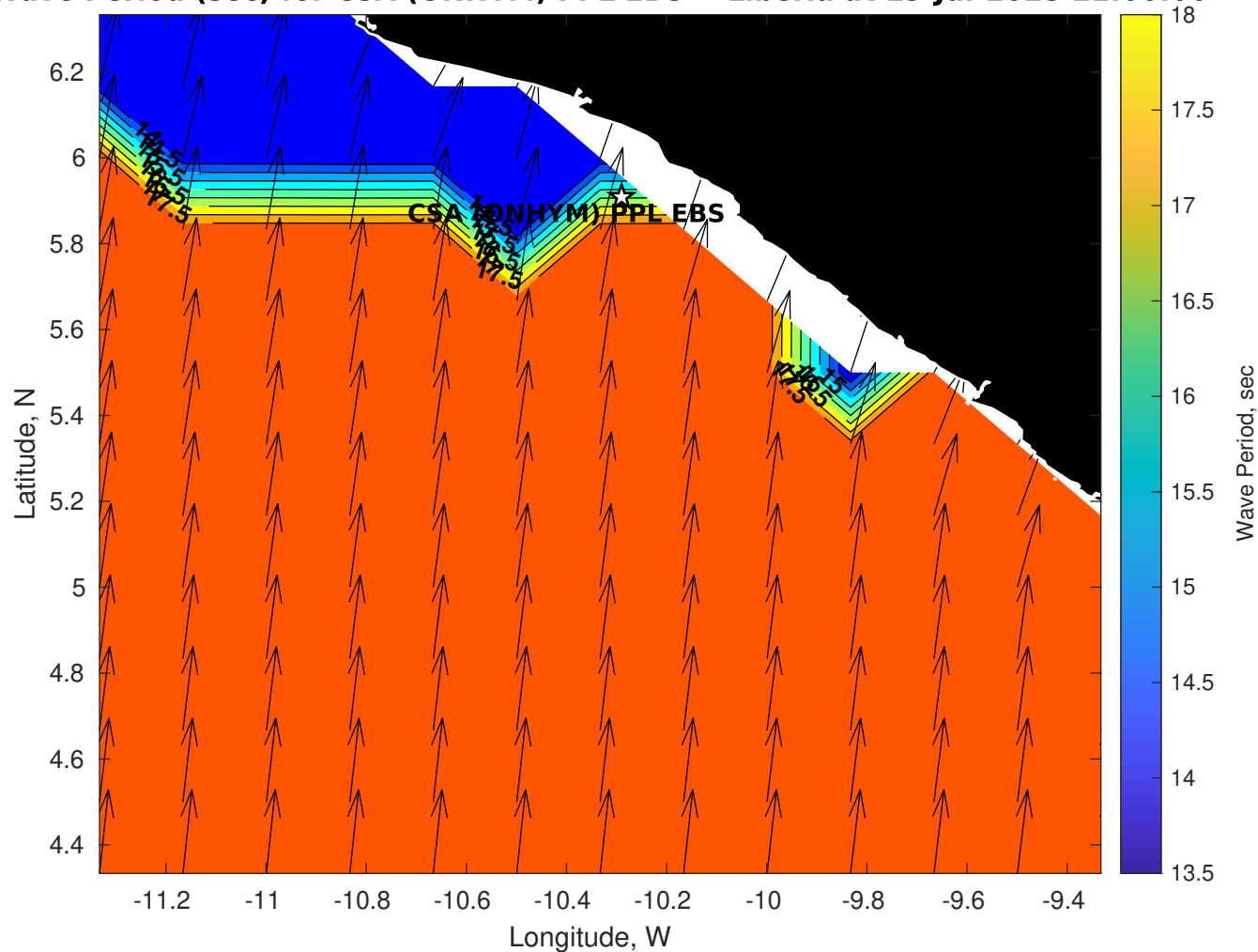
Wave Period (sec) for CSA (ONHYM) PPL EBS - Liberia at 19-Jul-2025 21:00:00
