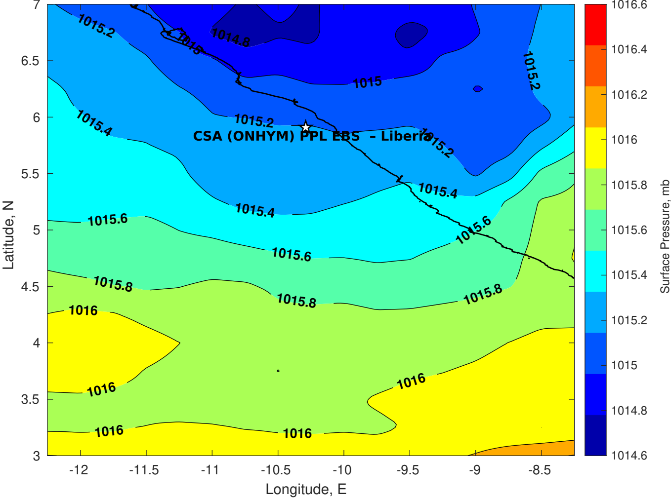
Surface Pressure (mb) for CSA (ONHYM) PPL EBS - Liberia at 21-Jul-2025 12:00:00
