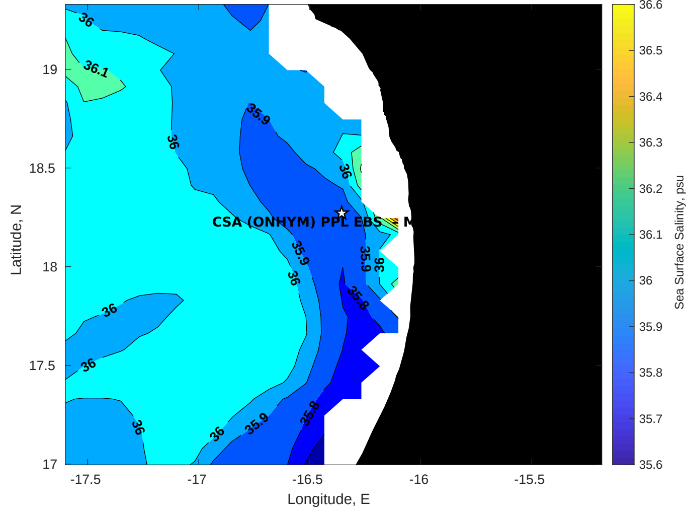
Surface Salinity for CSA (ONHYM) PPL EBS - Mauritania at 19-Jul-2025 00:00:00
