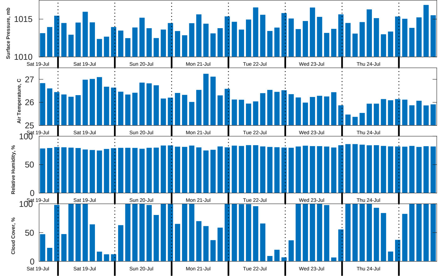
Met Forecast for CSA (ONHYM) PPL EBS - Nigeria from 19-Jul-2025 12:00:00 to 26-Jul-2025 12:00:00
