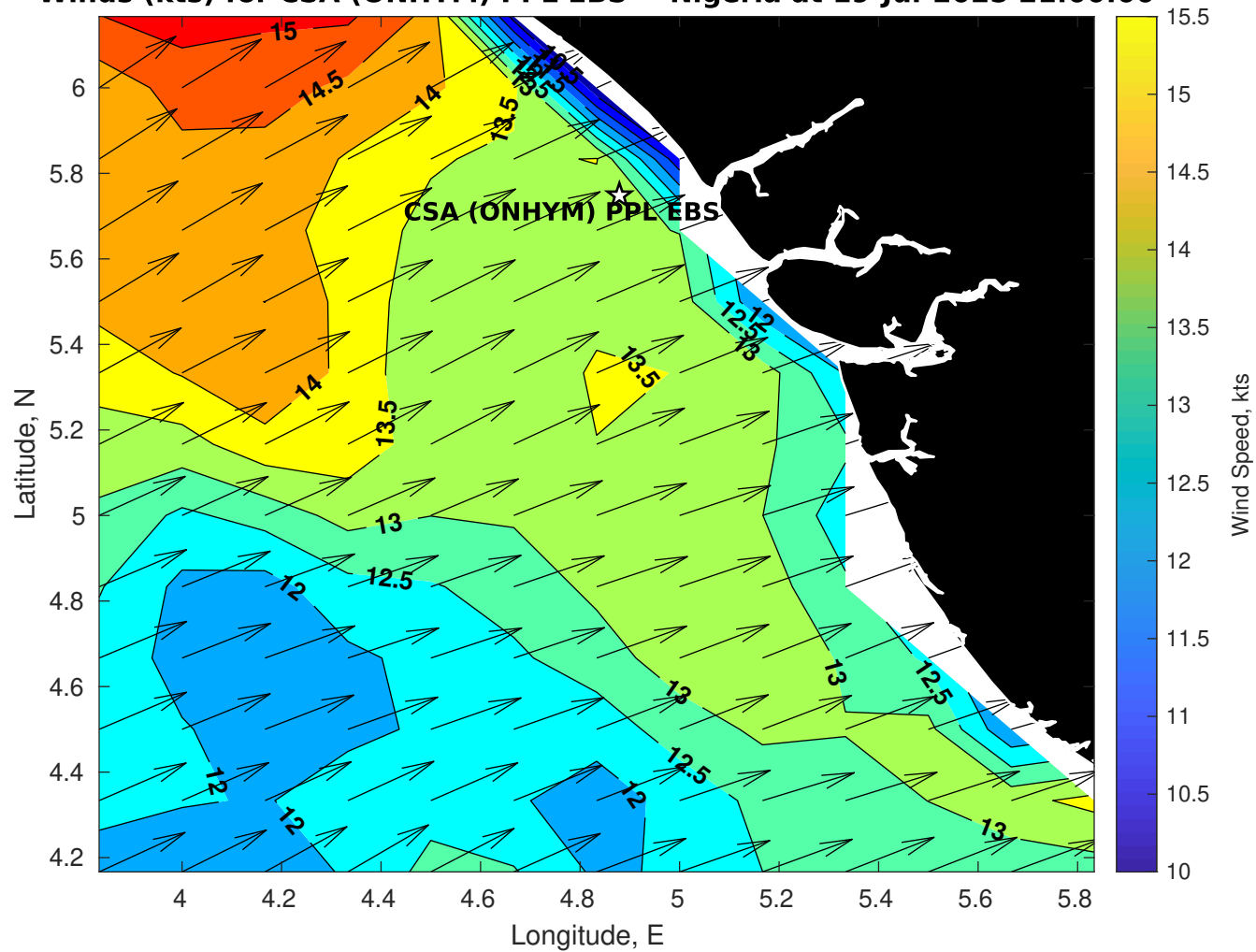
Winds (kts) for CSA (ONHYM) PPL EBS - Nigeria at 19-Jul-2025 21:00:00
