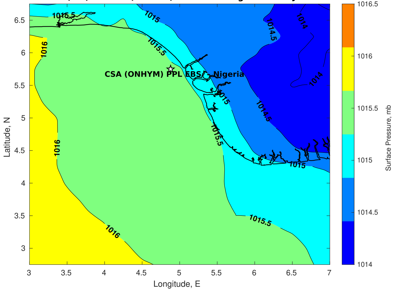
Surface Pressure (mb) for CSA (ONHYM) PPL EBS - Nigeria at 19-Jul-2025 12:00:00
