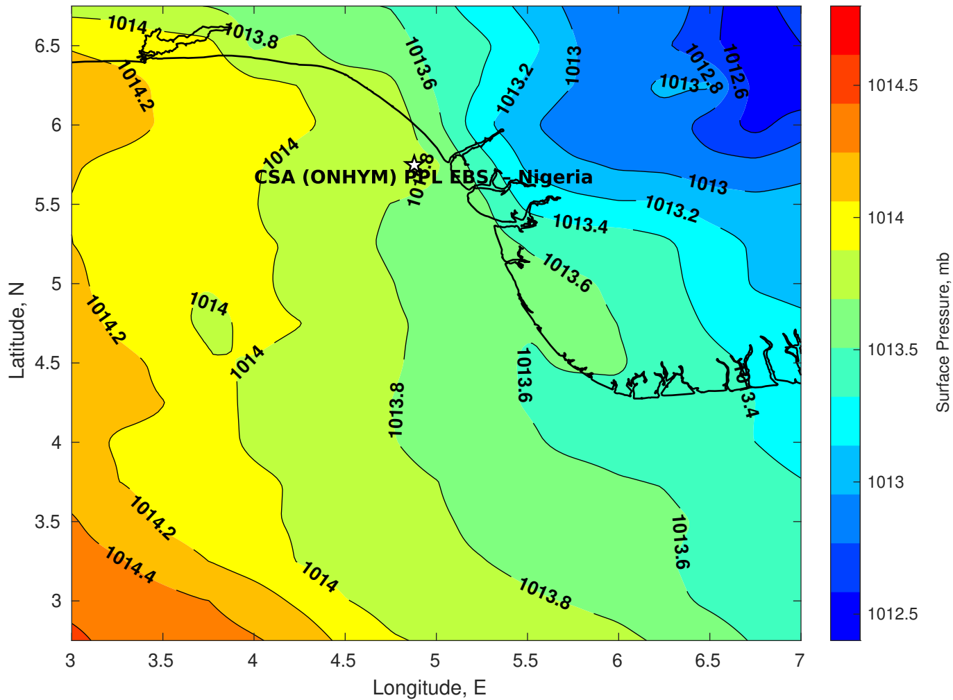
Surface Pressure (mb) for CSA (ONHYM) PPL EBS - Nigeria at 21-Jul-2025 12:00:00
