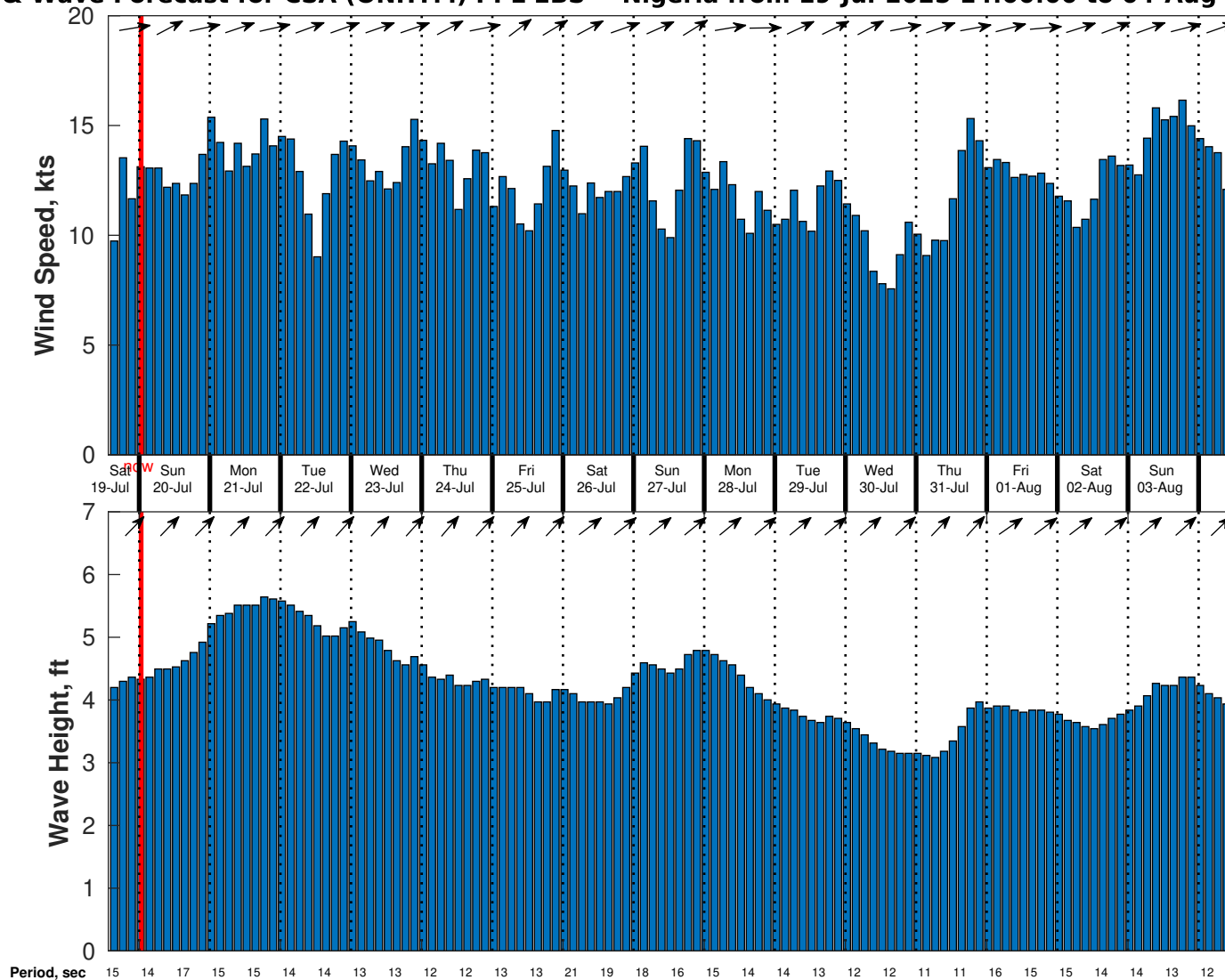
Wind & Wave Forecast for CSA (ONHYM) PPL EBS - Nigeria from 19-Jul-2025 14:00:00 to 04-Aug-2025 14:00:00
