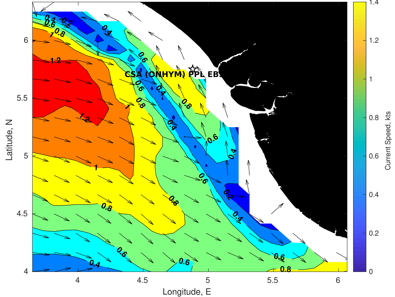
Surface Currents for CSA (ONHYM) PPL EBS - Nigeria at 19-Jul-2025 00:00:00
