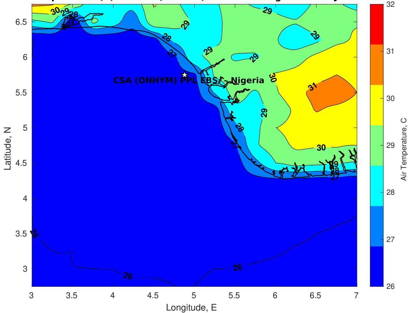
Air Temperature (C) for CSA (ONHYM) PPL EBS - Nigeria at 19-Jul-2025
