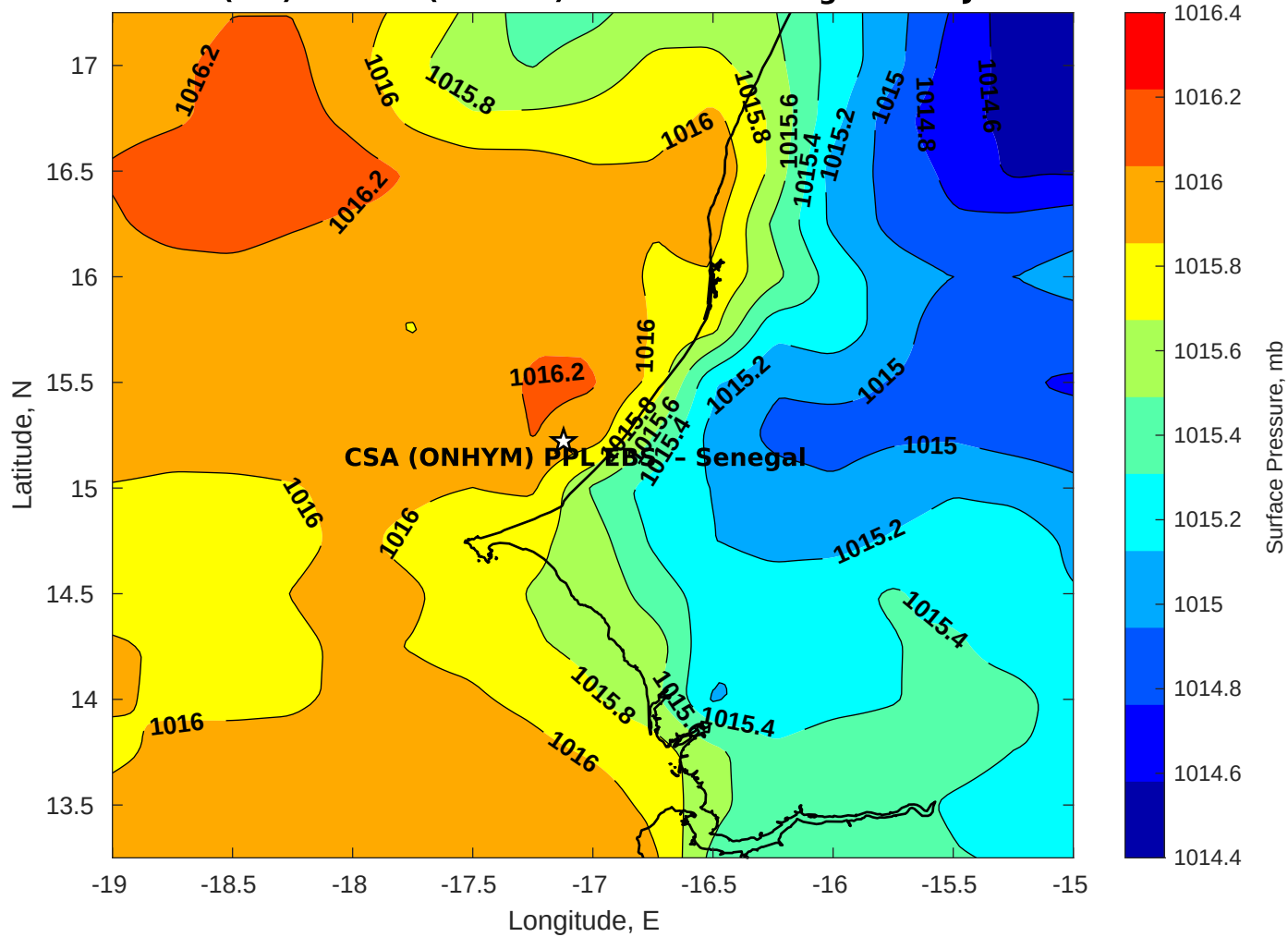
Surface Pressure (mb) for CSA (ONHYM) PPL EBS - Senegal at 19-Jul-2025 12:00:00
