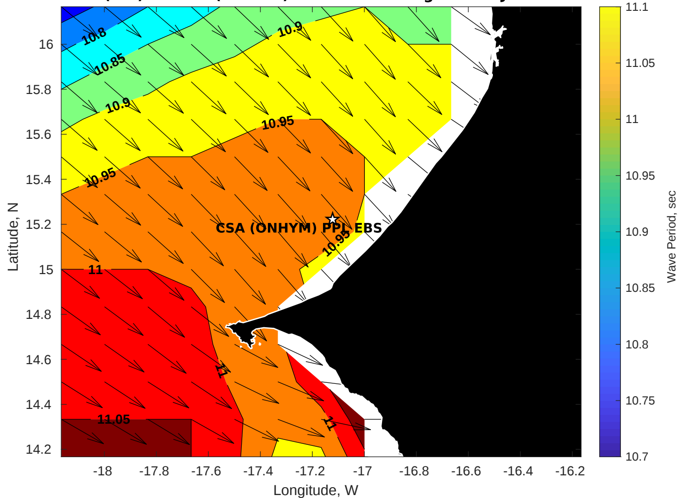
Wave Period (sec) for CSA (ONHYM) PPL EBS - Senegal at 19-Jul-2025 21:00:00
