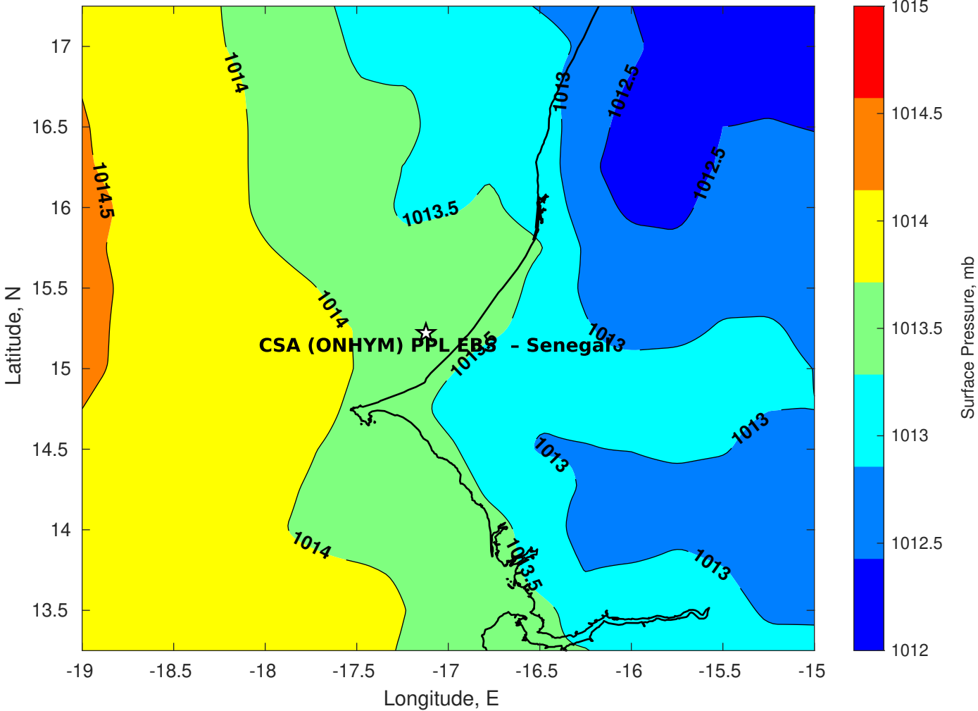
Surface Pressure (mb) for CSA (ONHYM) PPL EBS - Senegal at 21-Jul-2025 12:00:00
