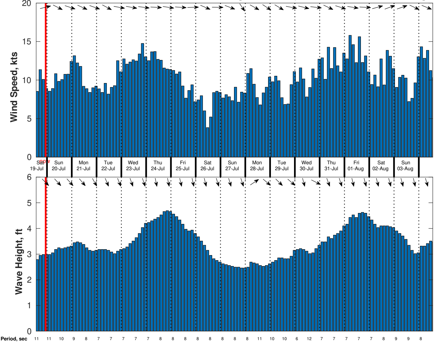
Wind & Wave Forecast for CSA (ONHYM) PPL EBS - Senegal from 19-Jul-2025 13:00:00 to 04-Aug-2025 13:00:00
