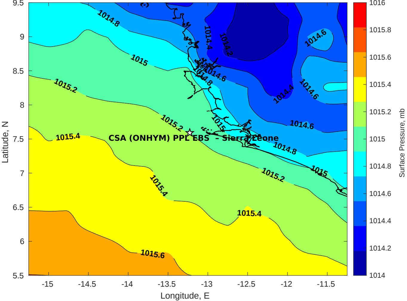
Surface Pressure (mb) for CSA (ONHYM) PPL EBS - Sierra Leone at 21-Jul-2025 12:00:00
