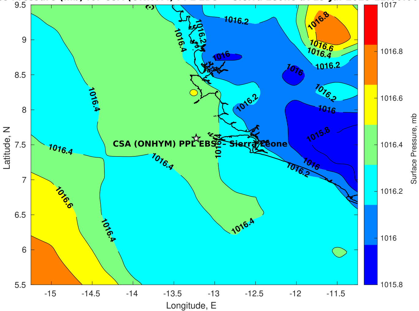
Surface Pressure (mb) for CSA (ONHYM) PPL EBS - Sierra Leone at 19-Jul-2025 12:00:00
