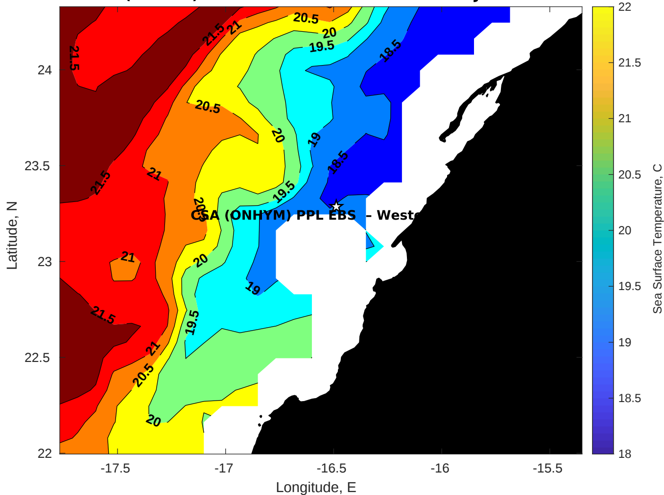
SST for CSA (ONHYM) PPL EBS - Western Sahara at 19-Jul-2025 00:00:00
