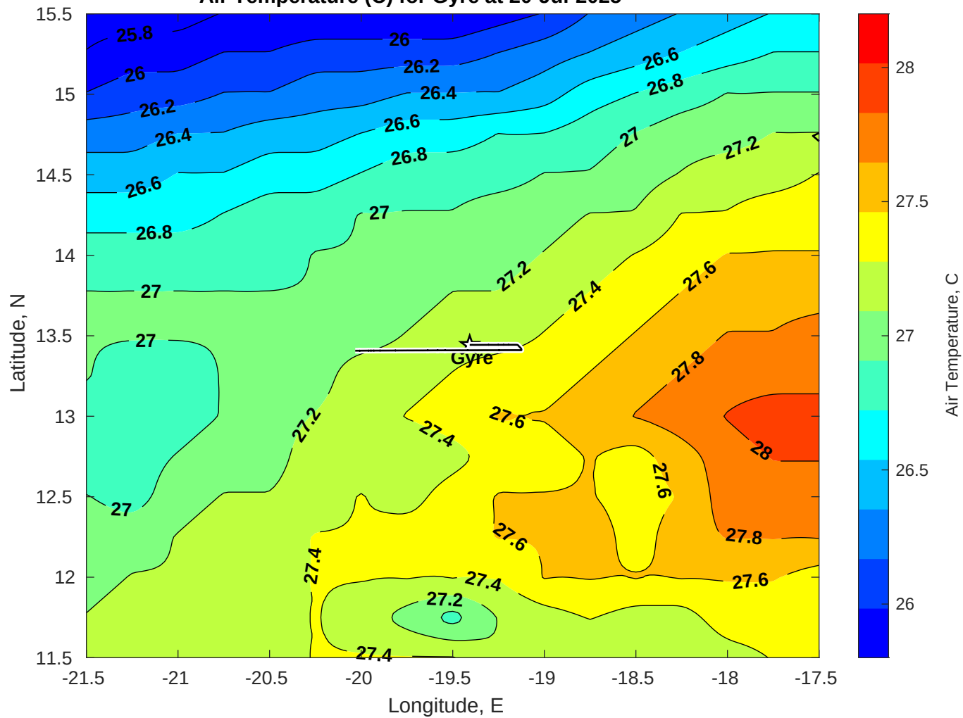
Air Temperature (C) for Gyre at 20-Jul-2025
