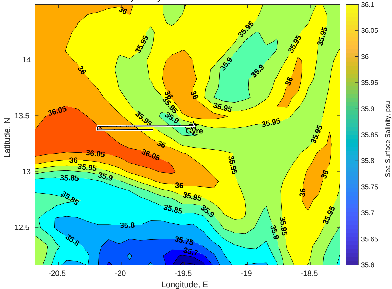
Surface Salinity for Gyre at 19-Jul-2025 00:00:00
