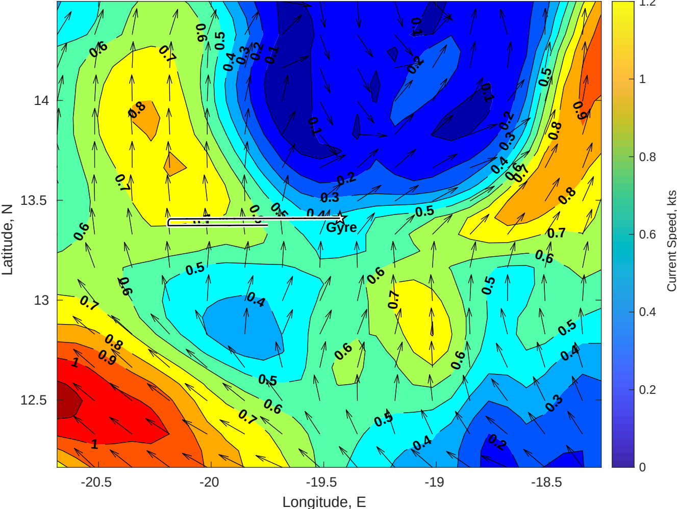
Surface Currents for Gyre at 19-Jul-2025 00:00:00
