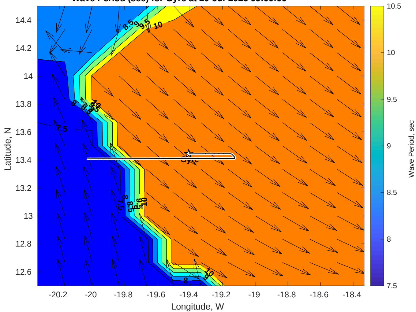
Wave Period (sec) for Gyre at 20-Jul-2025 09:00:00
