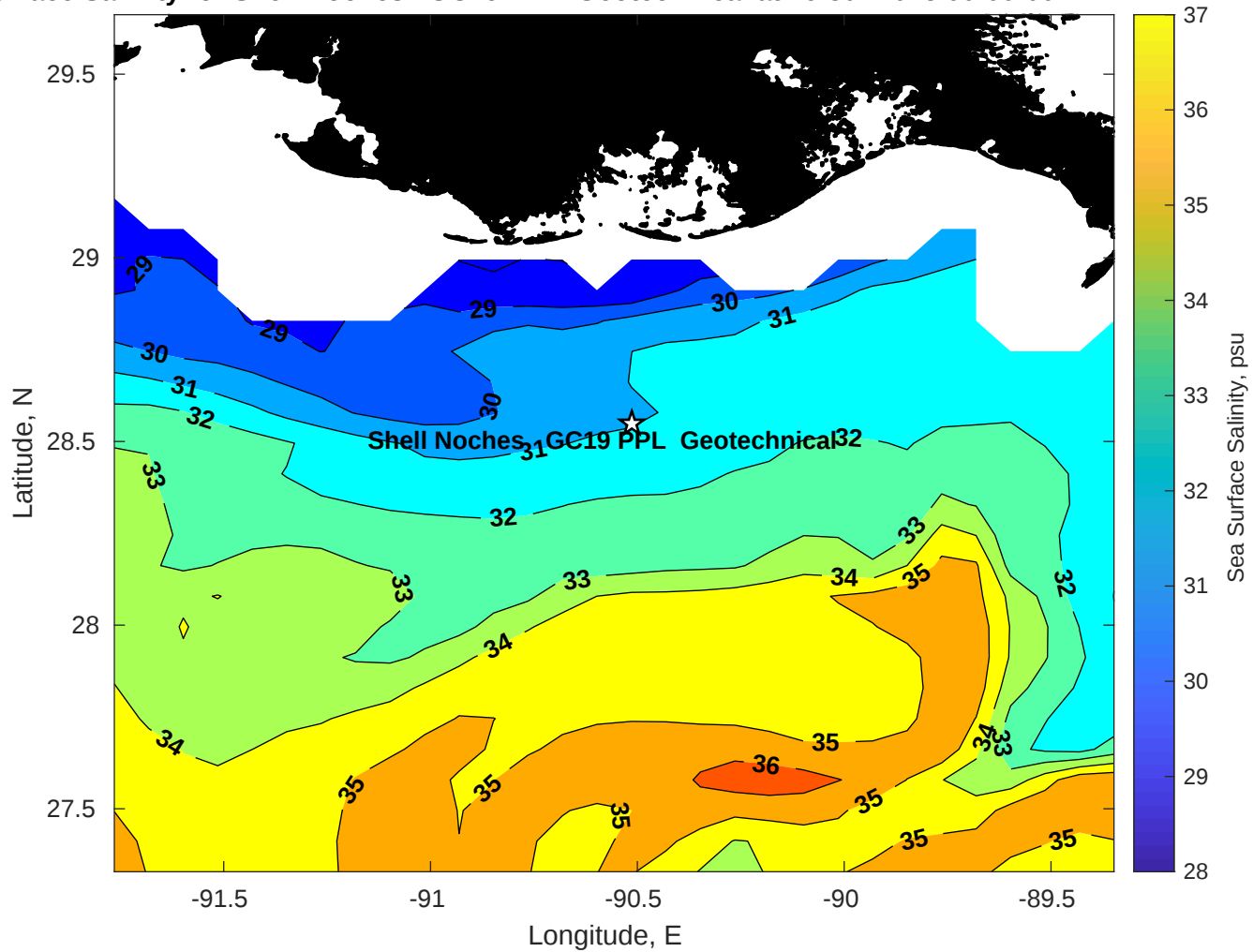
Surface Salinity for Shell Noches GC19 PPL Geotechnical at 19-Jul-2025 00:00:00
