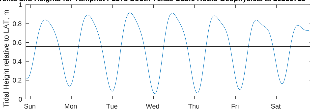
Tidal Currents and Heights for Tampnet P2378 South Texas Cable Route Geophysical at 20250719
