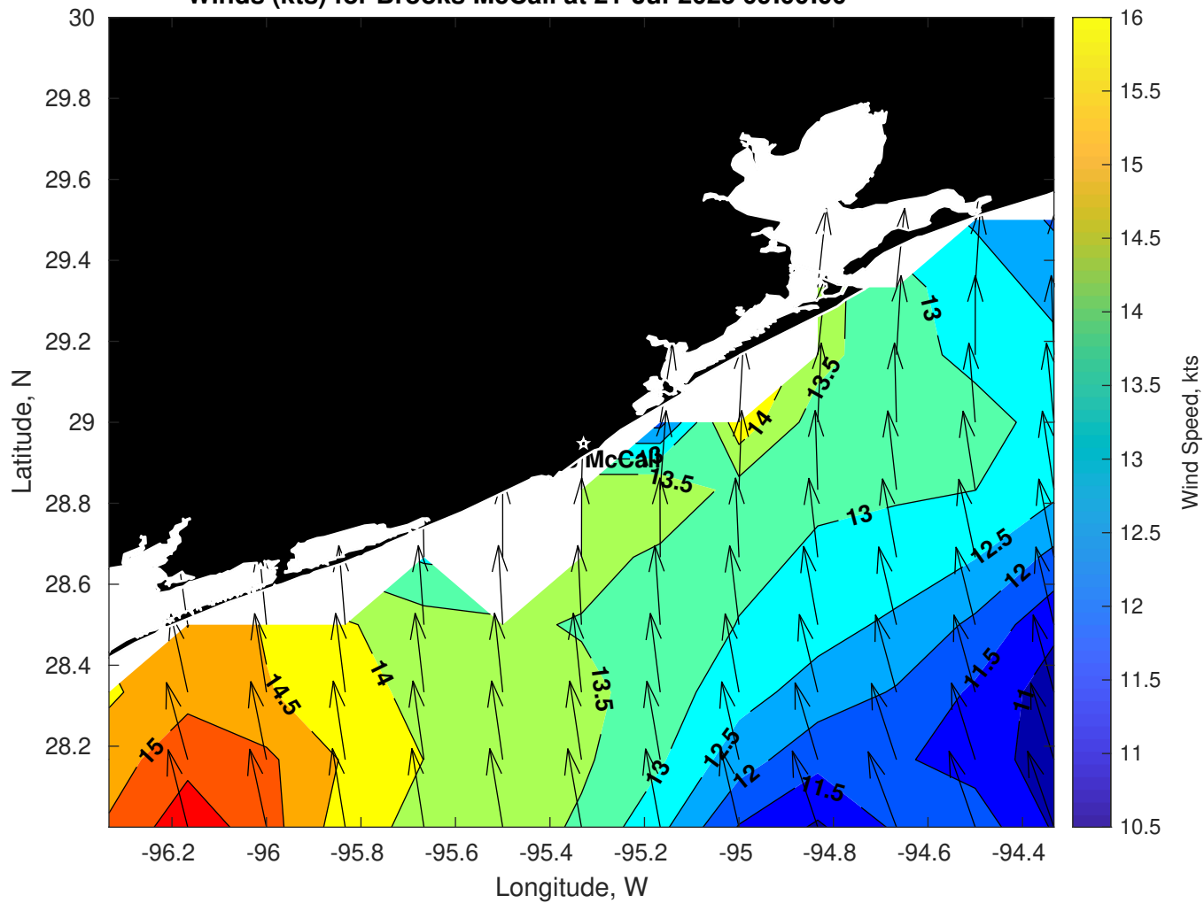
Winds (kts) for Brooks McCall at 21-Jul-2025 09:00:00
