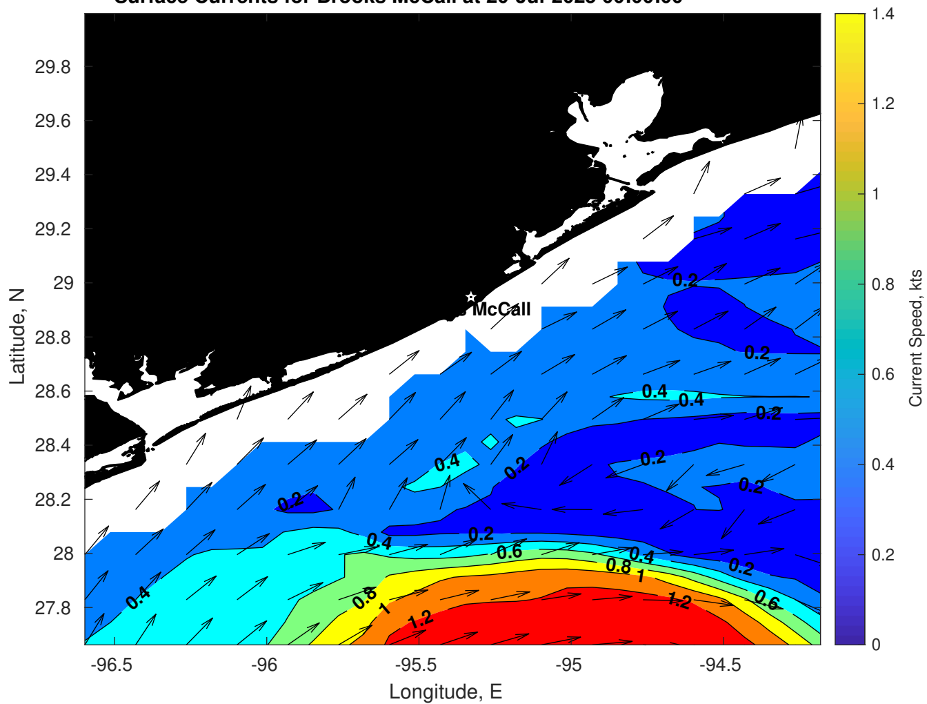
Surface Currents for Brooks McCall at 20-Jul-2025 00:00:00
