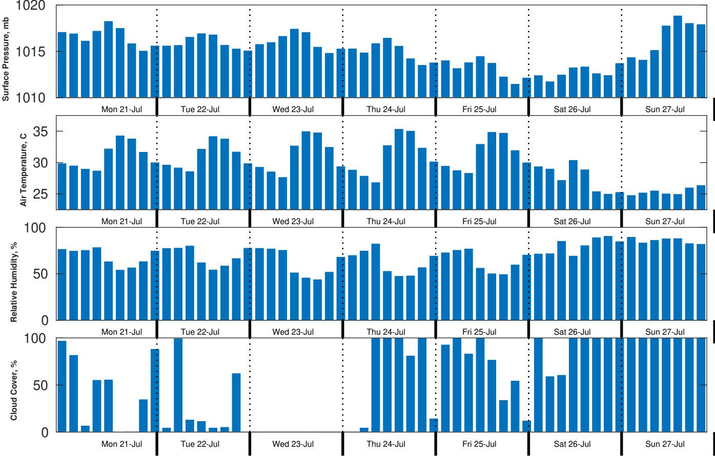
Met Forecast for Brooks McCall from 21-Jul-2025 00:00:00 to 28-Jul-2025 00:00:00
