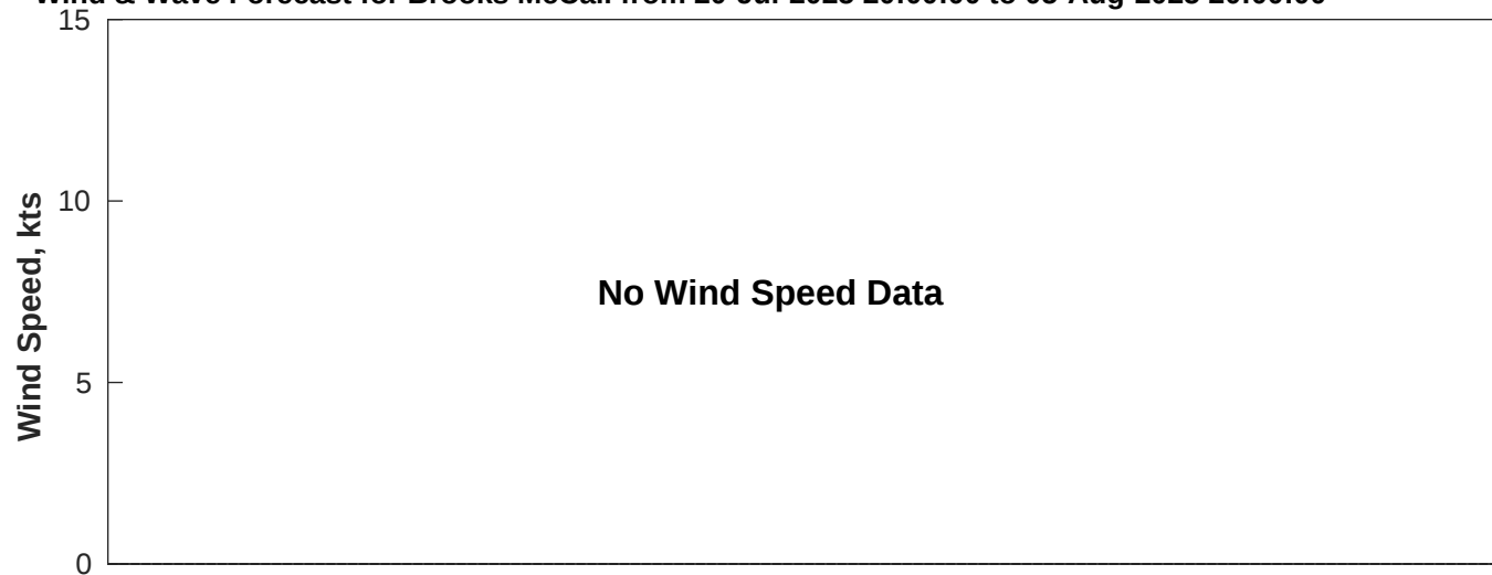
Wind & Wave Forecast for Brooks McCall from 20-Jul-2025 20:00:00 to 05-Aug-2025 20:00:00
