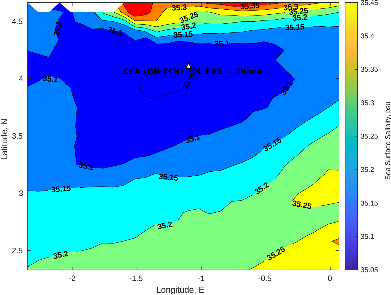
Surface Salinity for CSA (ONHYM) PPL EBS - Ghana at 19-Jul-2025 00:00:00
