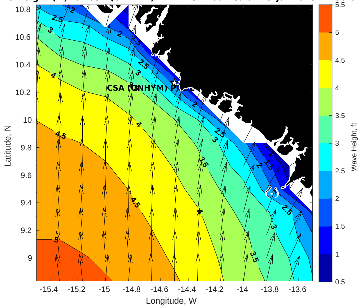
Wave Height (ft) for CSA (ONHYM) PPL EBS - Guinea at 19-Jul-2025 21:00:00
