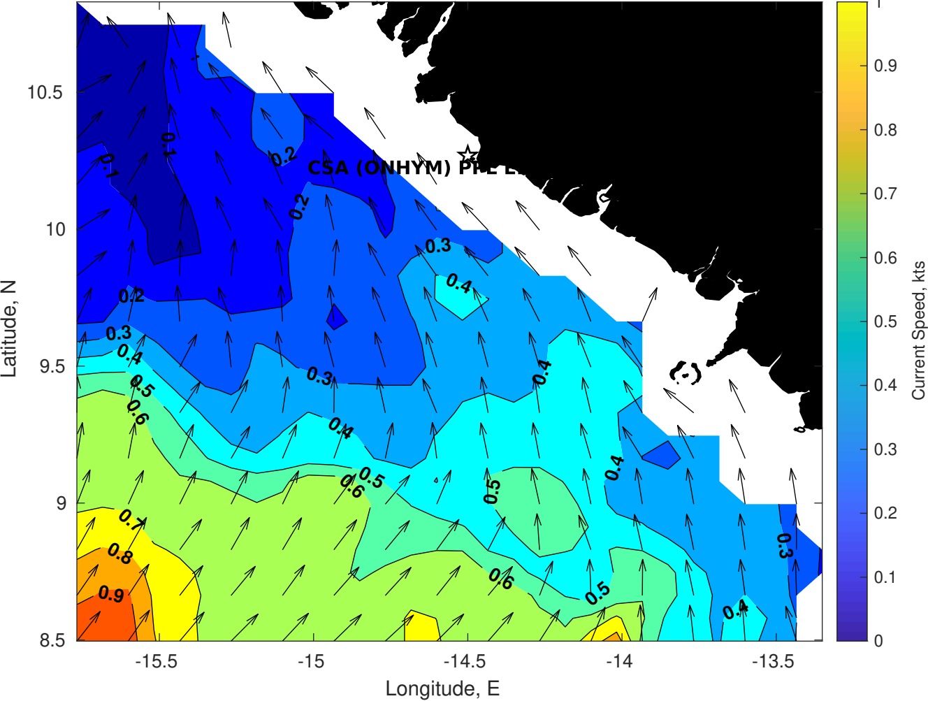
Surface Currents for CSA (ONHYM) PPL EBS - Guinea at 19-Jul-2025 00:00:00
