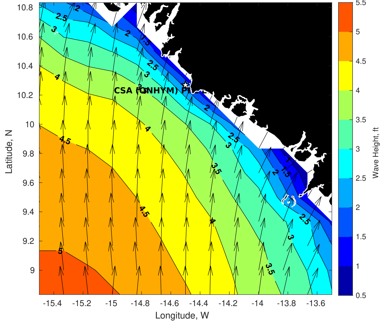
Wave Height (ft) for CSA (ONHYM) PPL EBS - Guinea at 19-Jul-2025 21:00:00
