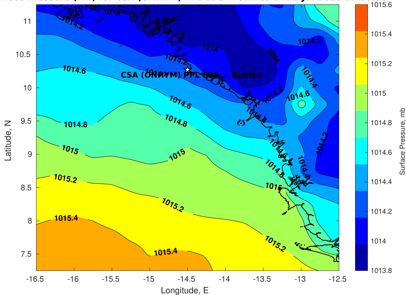
Surface Pressure (mb) for CSA (ONHYM) PPL EBS - Guinea at 21-Jul-2025 12:00:00
