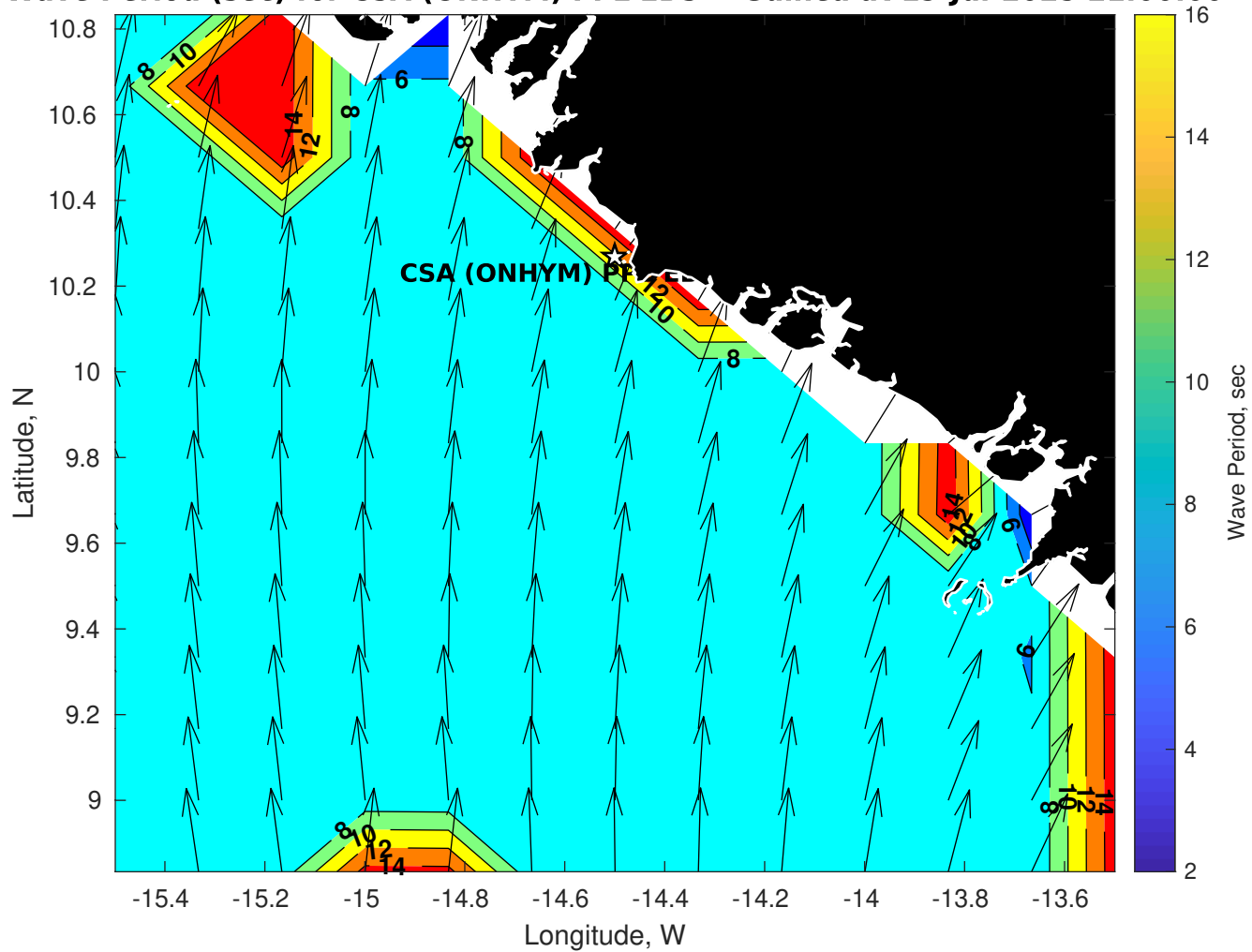
Wave Period (sec) for CSA (ONHYM) PPL EBS - Guinea at 19-Jul-2025 21:00:00
