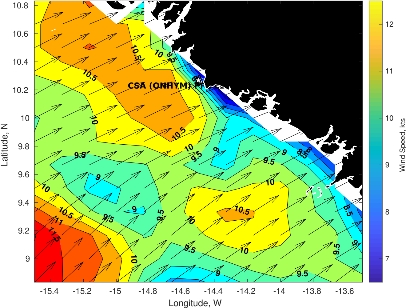
Winds (kts) for CSA (ONHYM) PPL EBS - Guinea at 19-Jul-2025 21:00:00
