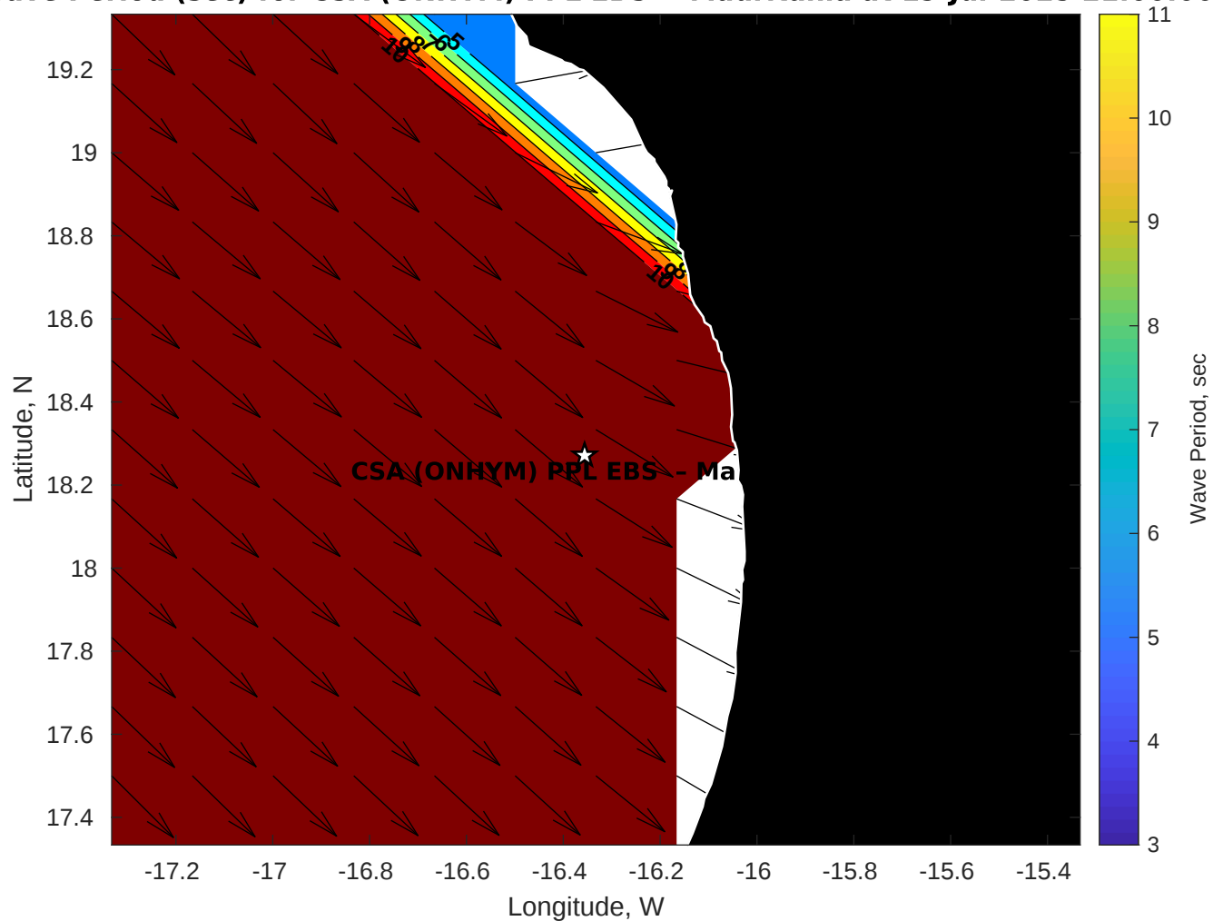
Wave Period (sec) for CSA (ONHYM) PPL EBS - Mauritania at 19-Jul-2025 21:00:00
