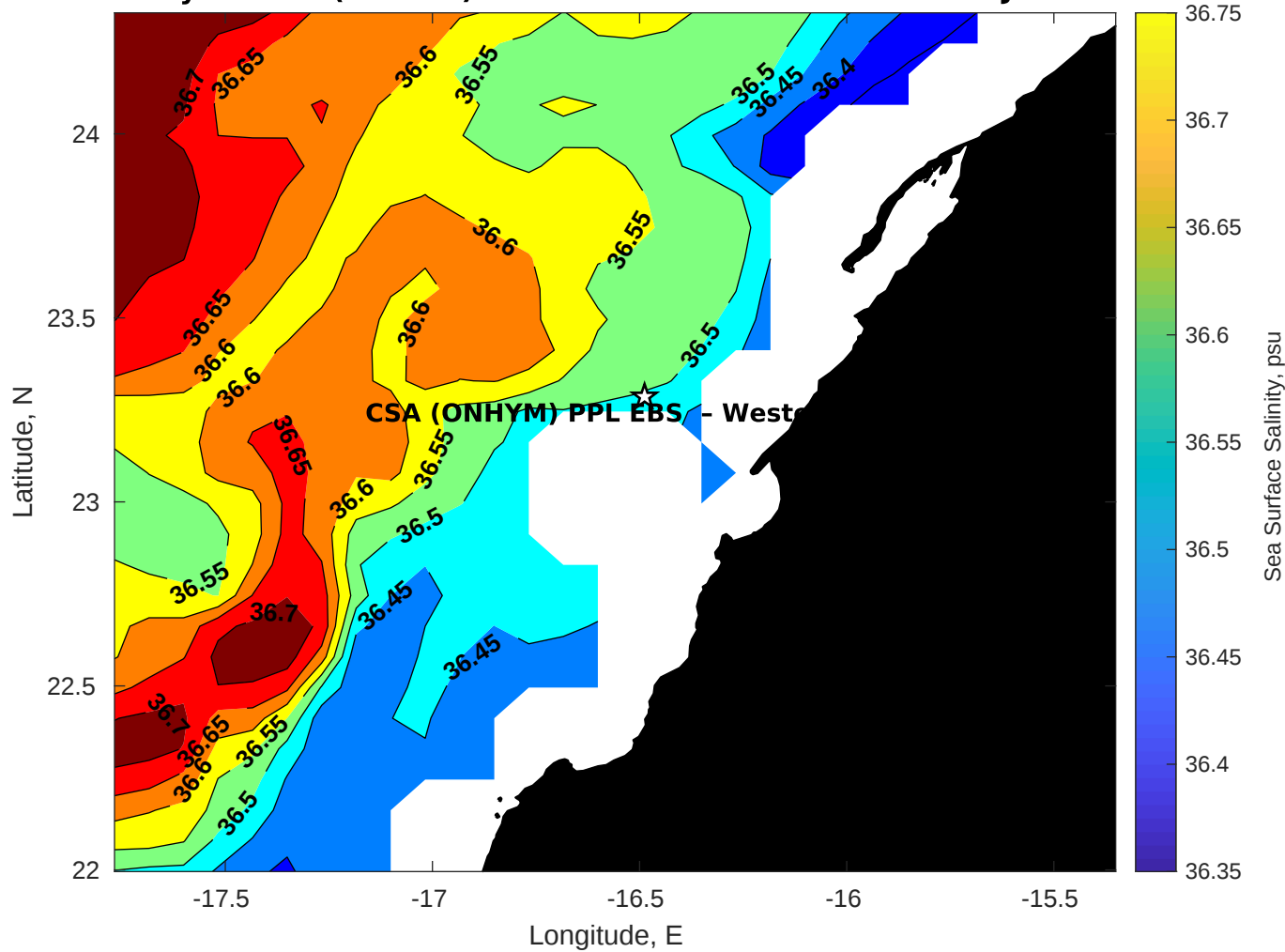
Surface Salinity for CSA (ONHYM) PPL EBS - Western Sahara at 19-Jul-2025 00:00:00
