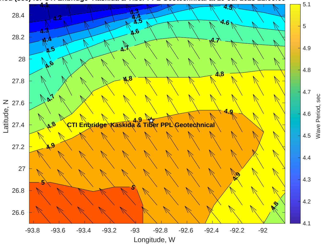
Wave Period (sec) for CTI Enbridge Kaskida & Tiber PPL Geotechnical at 19-Jul-2025 21:00:00
