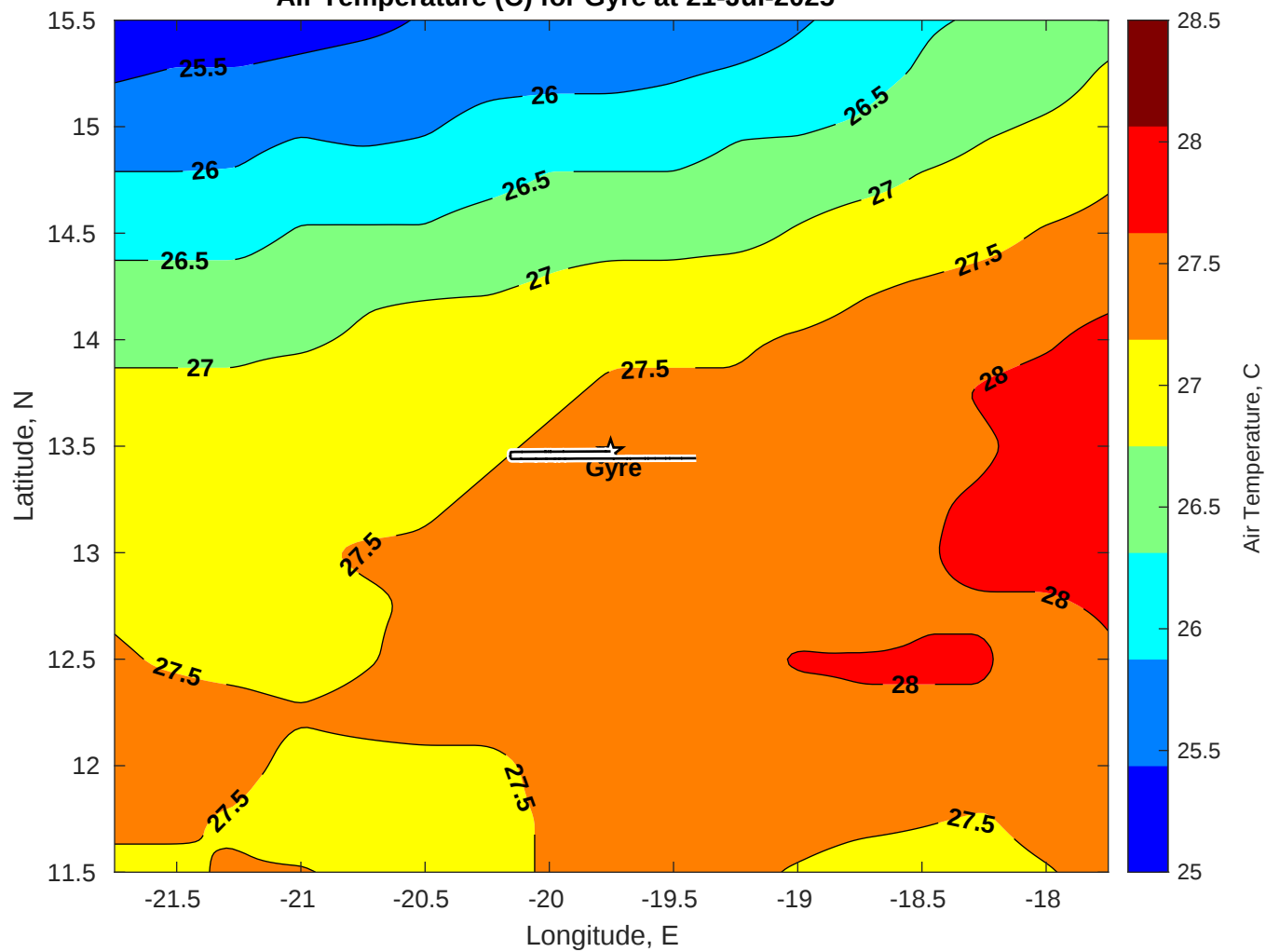
Air Temperature (C) for Gyre at 21-Jul-2025
