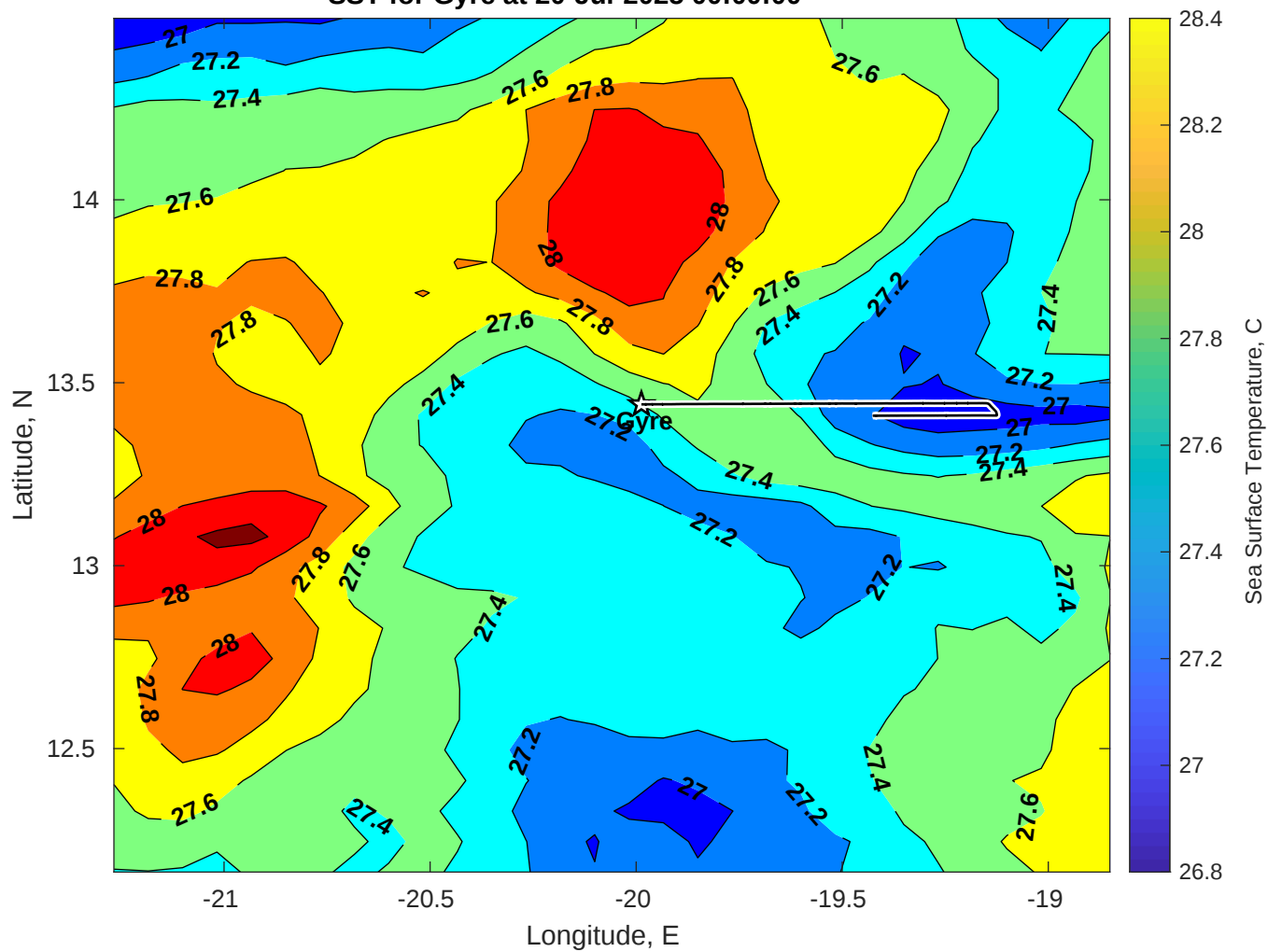
SST for Gyre at 20-Jul-2025 00:00:00
