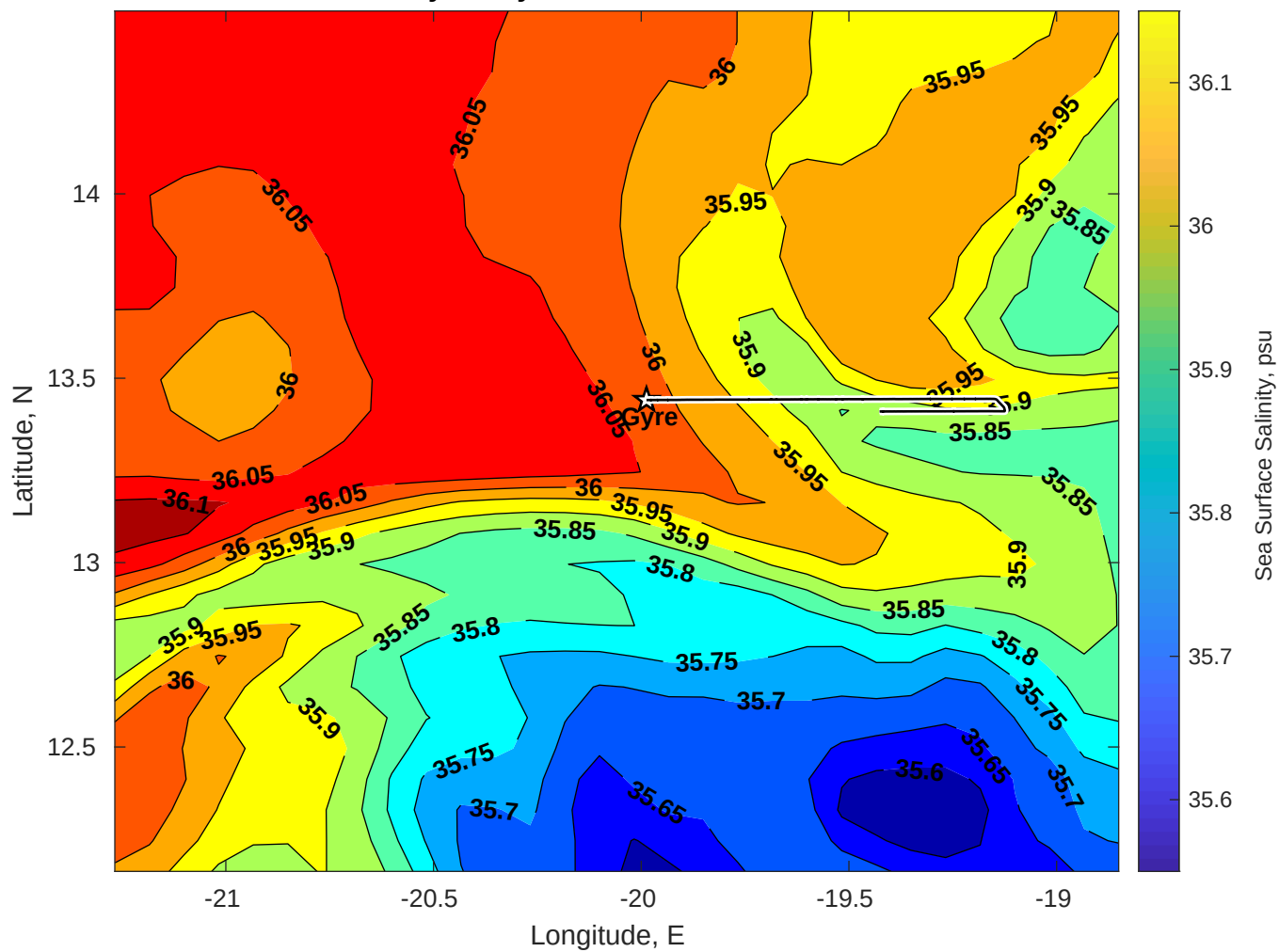
Surface Salinity for Gyre at 20-Jul-2025 00:00:00
