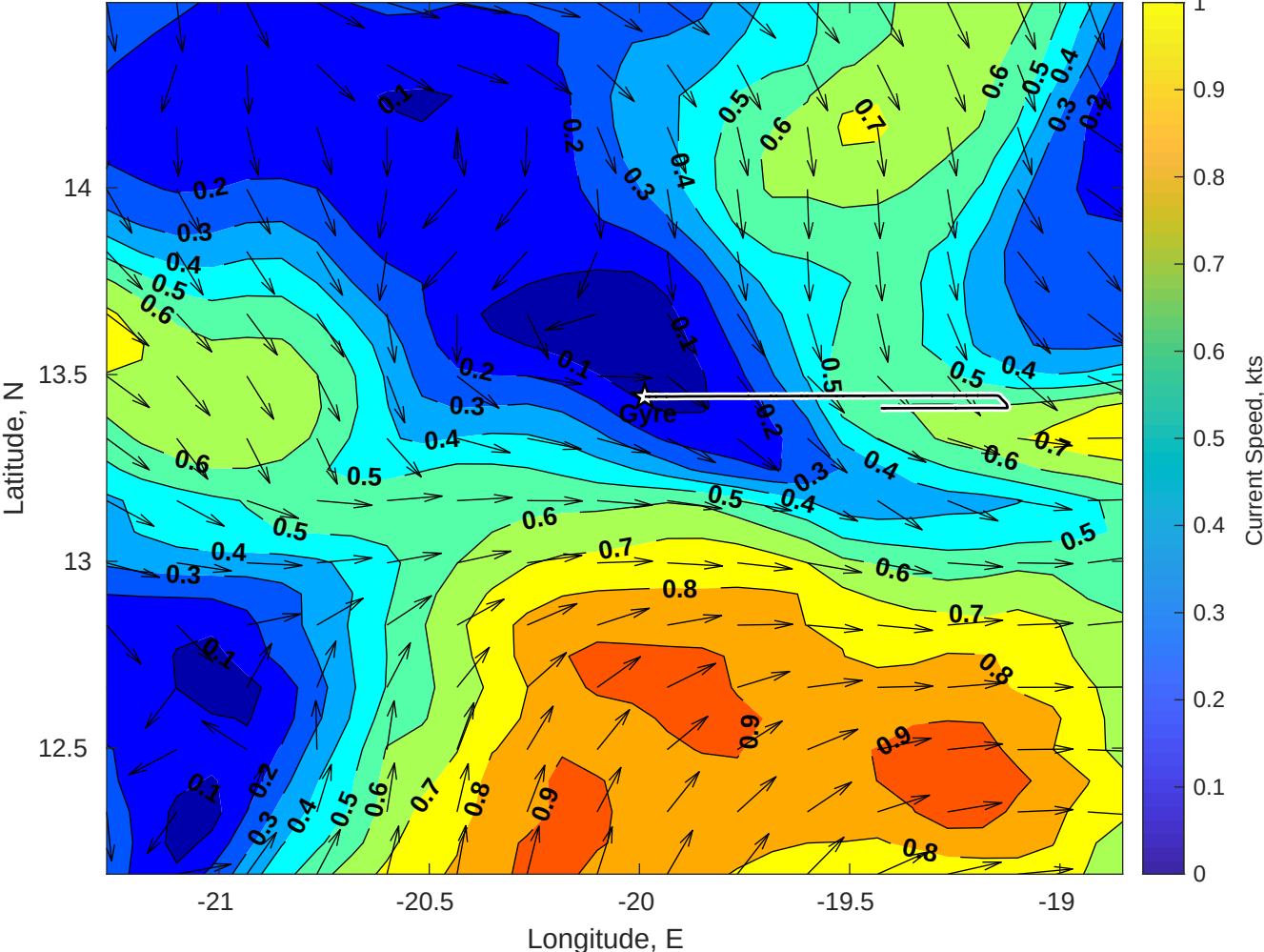
Surface Currents for Gyre at 20-Jul-2025 00:00:00
