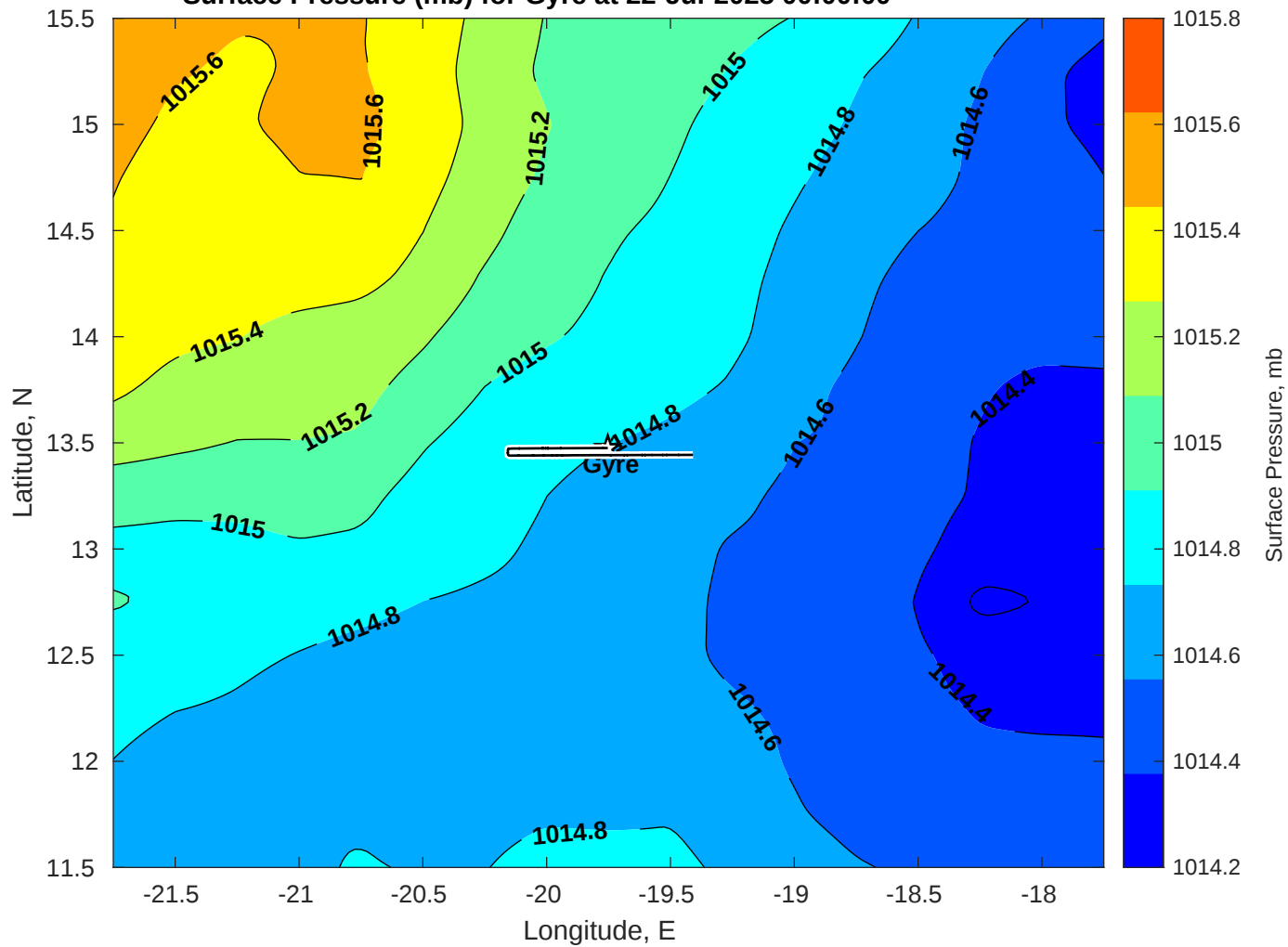
Surface Pressure (mb) for Gyre at 22-Jul-2025 00:00:00
