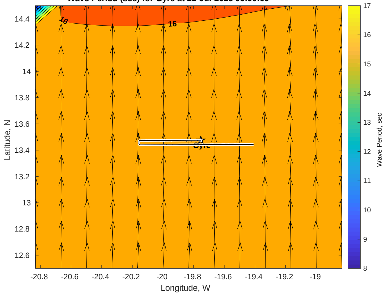
Wave Period (sec) for Gyre at 21-Jul-2025 09:00:00
