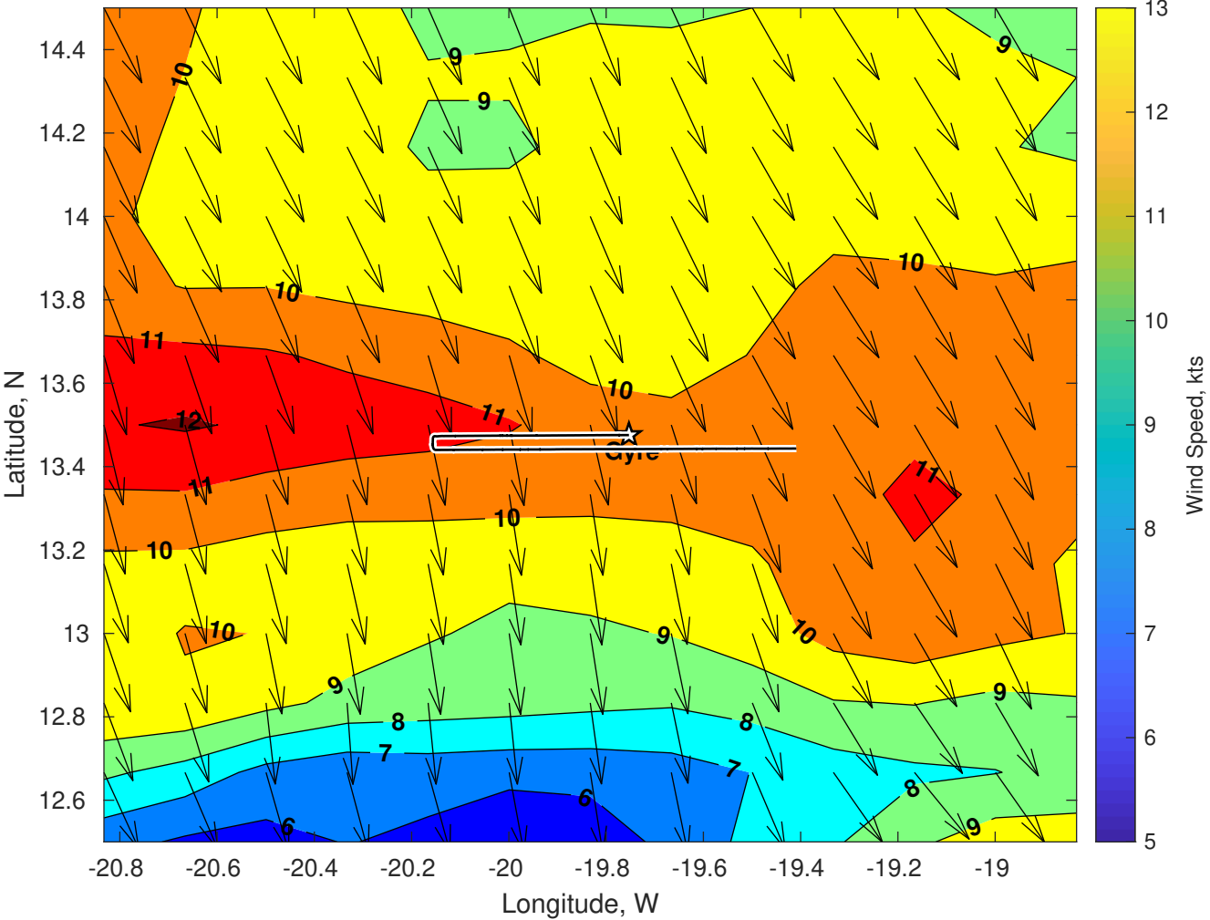
Winds (kts) for Gyre at 21-Jul-2025 09:00:00
