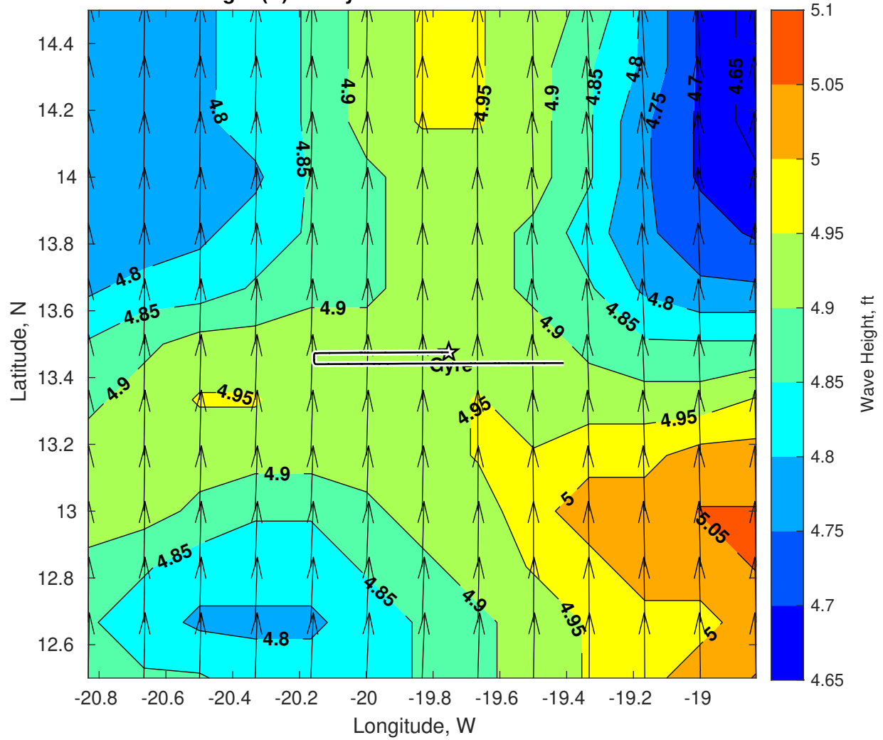
Wave Height (ft) for Gyre at 21-Jul-2025 09:00:00
