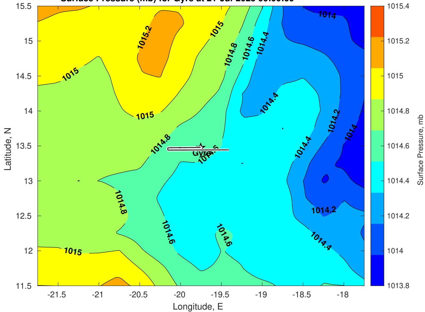
Surface Pressure (mb) for Gyre at 21-Jul-2025 00:00:00
