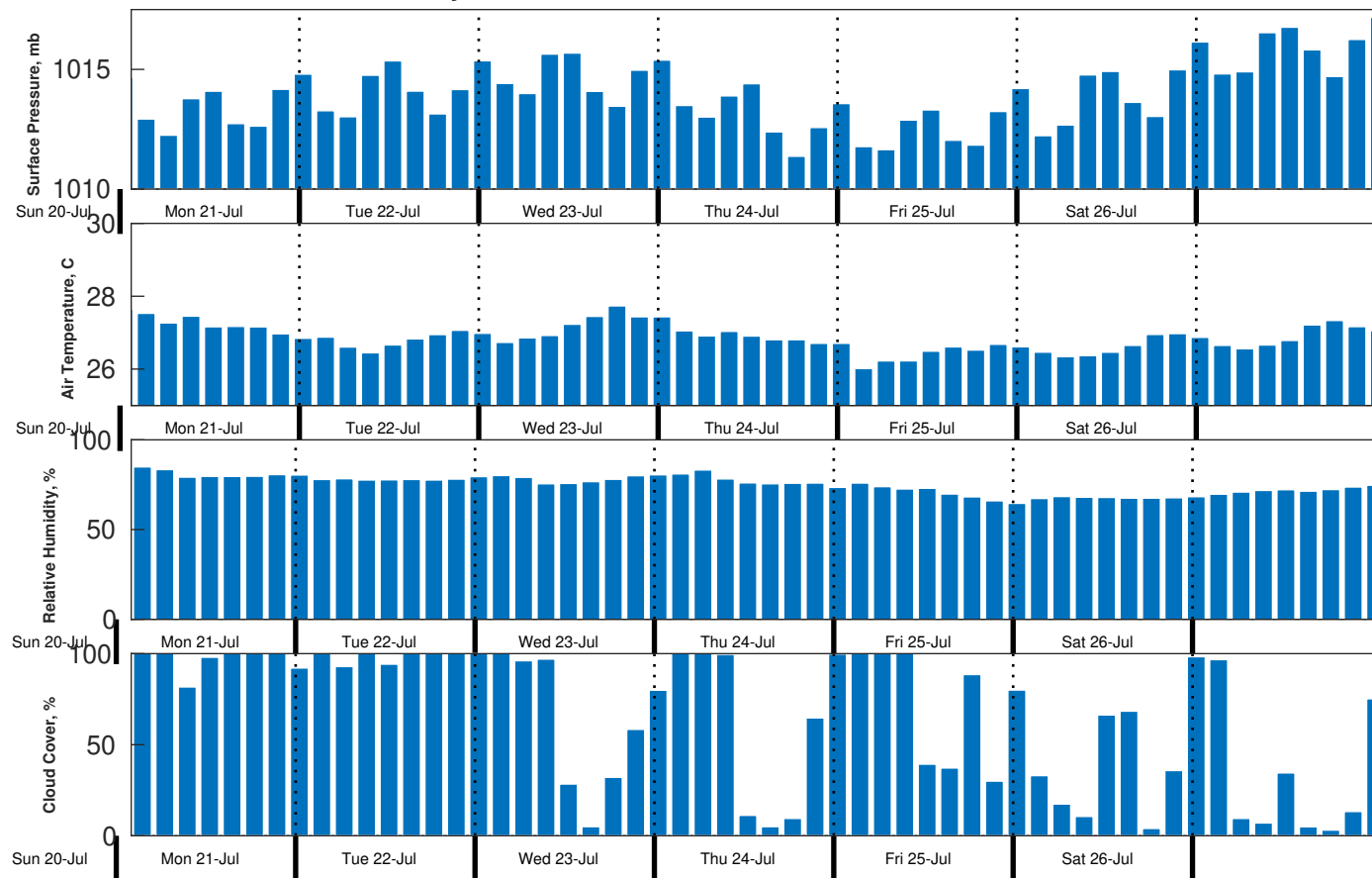
Met Forecast for Gyre from 20-Jul-2025 23:00:00 to 27-Jul-2025 23:00:00
