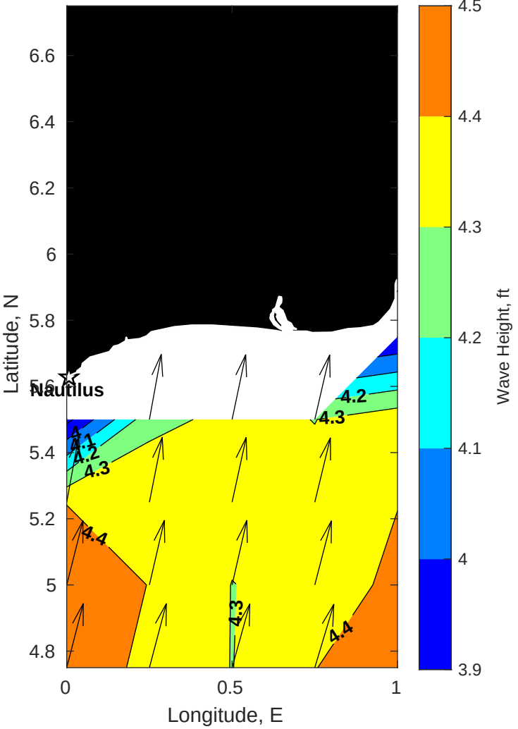
Wave Height (ft) for Nautilus at 19-Jul-2025 21:00:00
