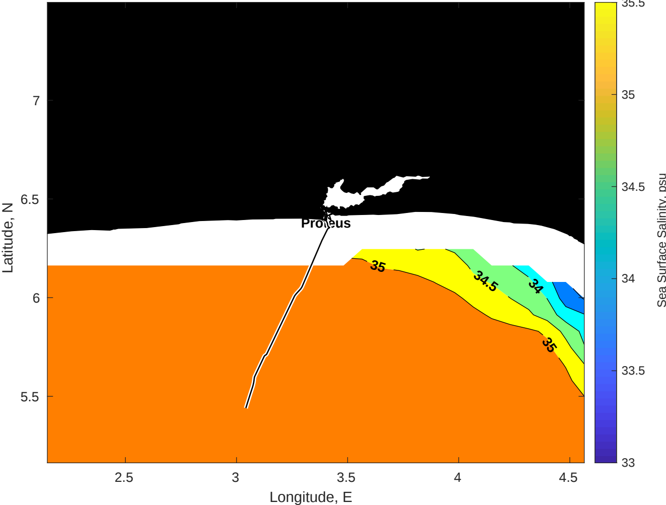
Surface Salinity for Proteus at 19-Jul-2025 00:00:00
