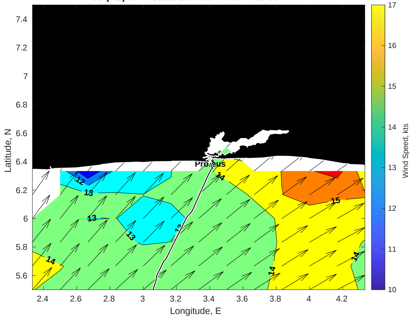
Winds (kts) for Proteus at 19-Jul-2025 21:00:00
