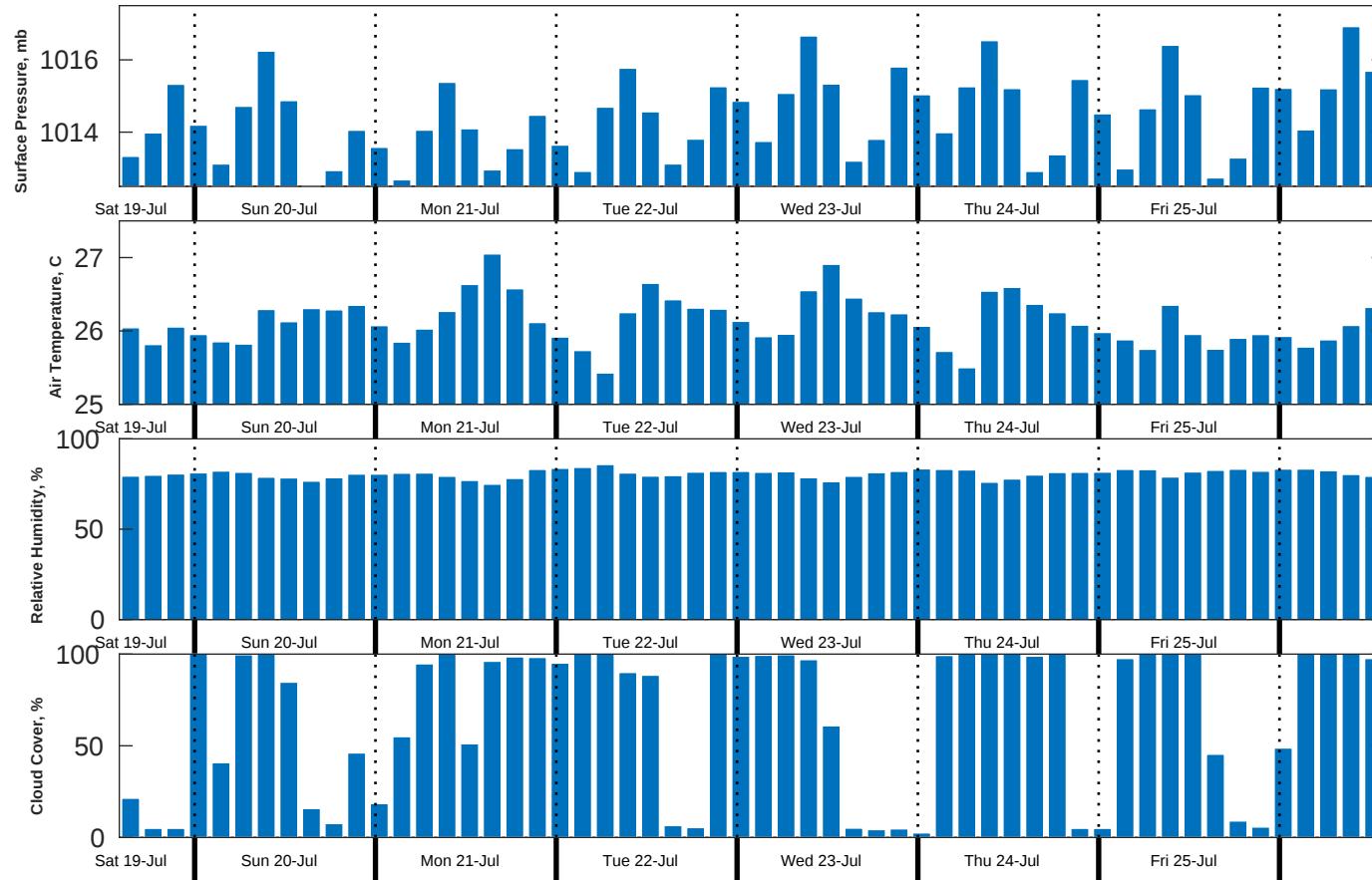
Met Forecast for Proteus from 19-Jul-2025 12:00:00 to 26-Jul-2025 12:00:00
