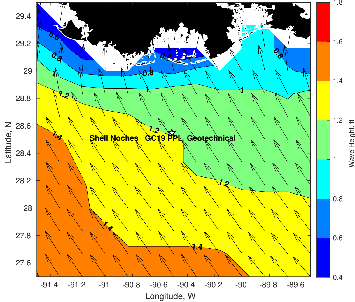
Wave Height (ft) for Shell Noches GC19 PPL Geotechnical at 19-Jul-2025 21:00:00
