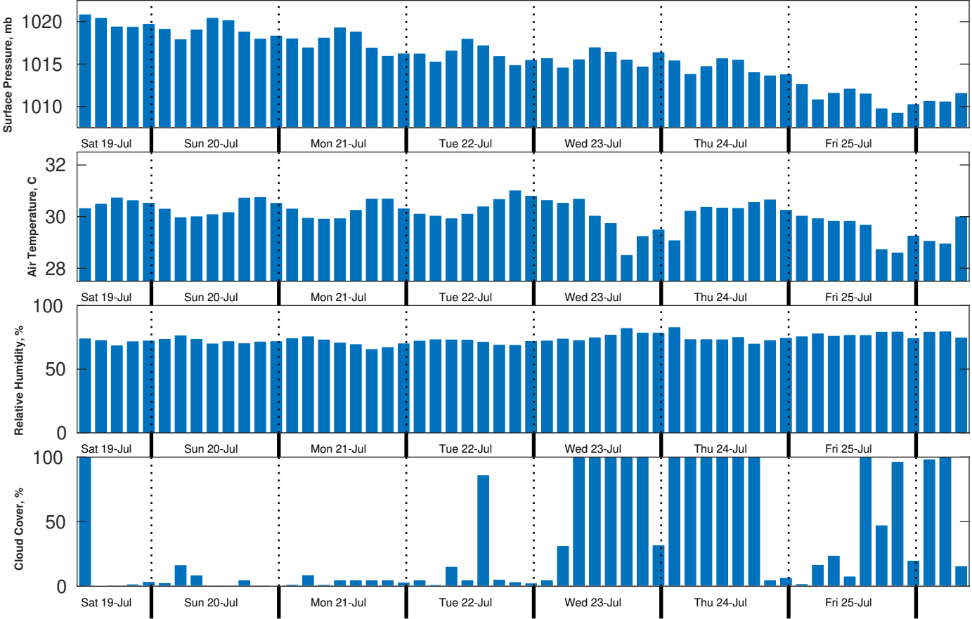
Met Forecast for Shell Noches GC19 PPL Geotechnical from 19-Jul-2025 12:00:00 to 26-Jul-2025 12:00:00
