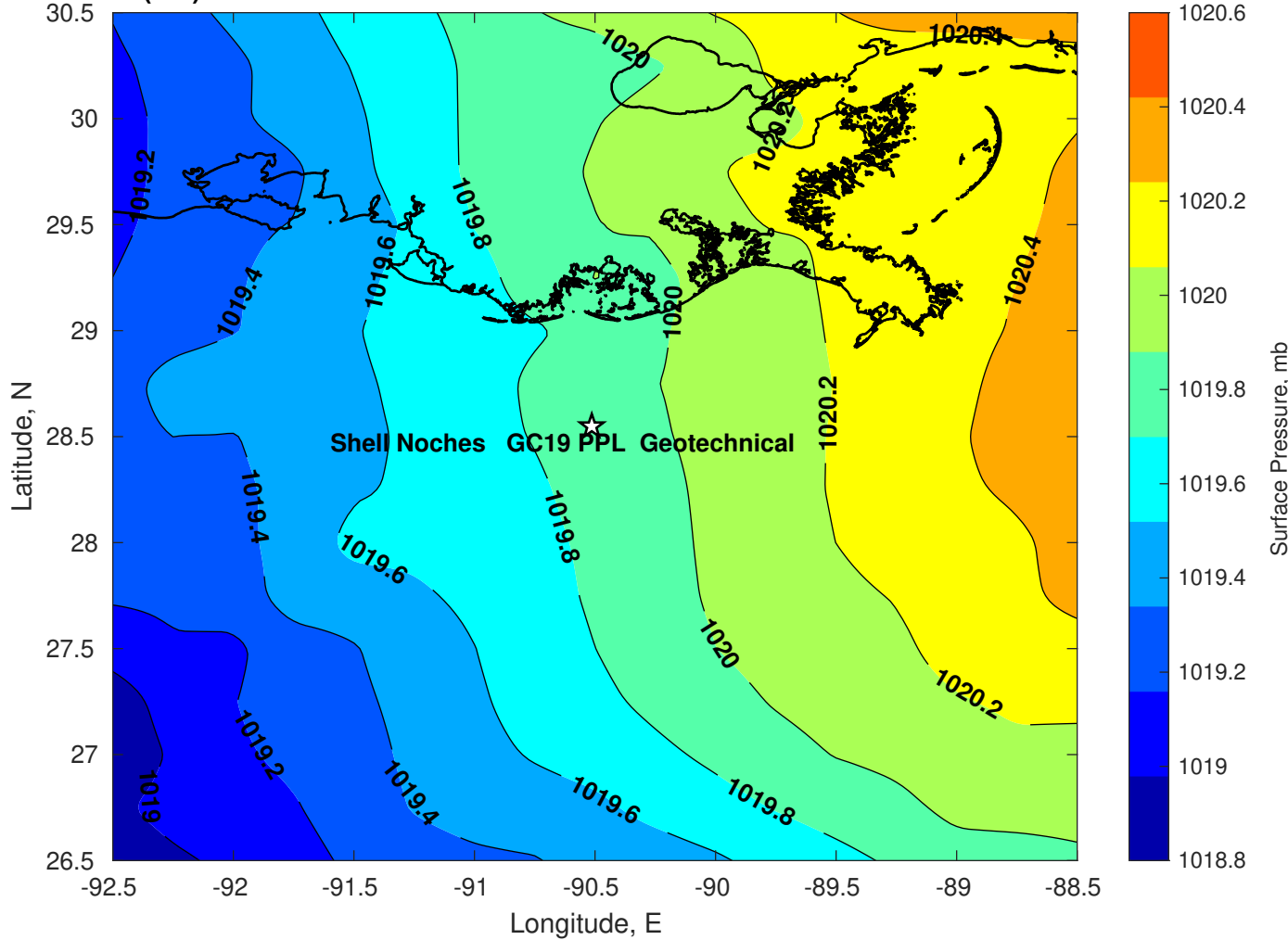
Surface Pressure (mb) for Shell Noches GC19 PPL Geotechnical at 19-Jul-2025 12:00:00
