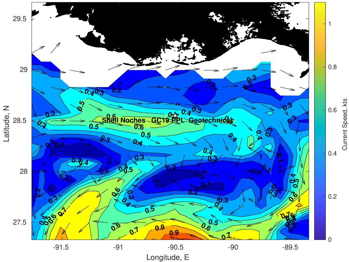
Surface Currents for Shell Noches GC19 PPL Geotechnical at 19-Jul-2025 00:00:00
