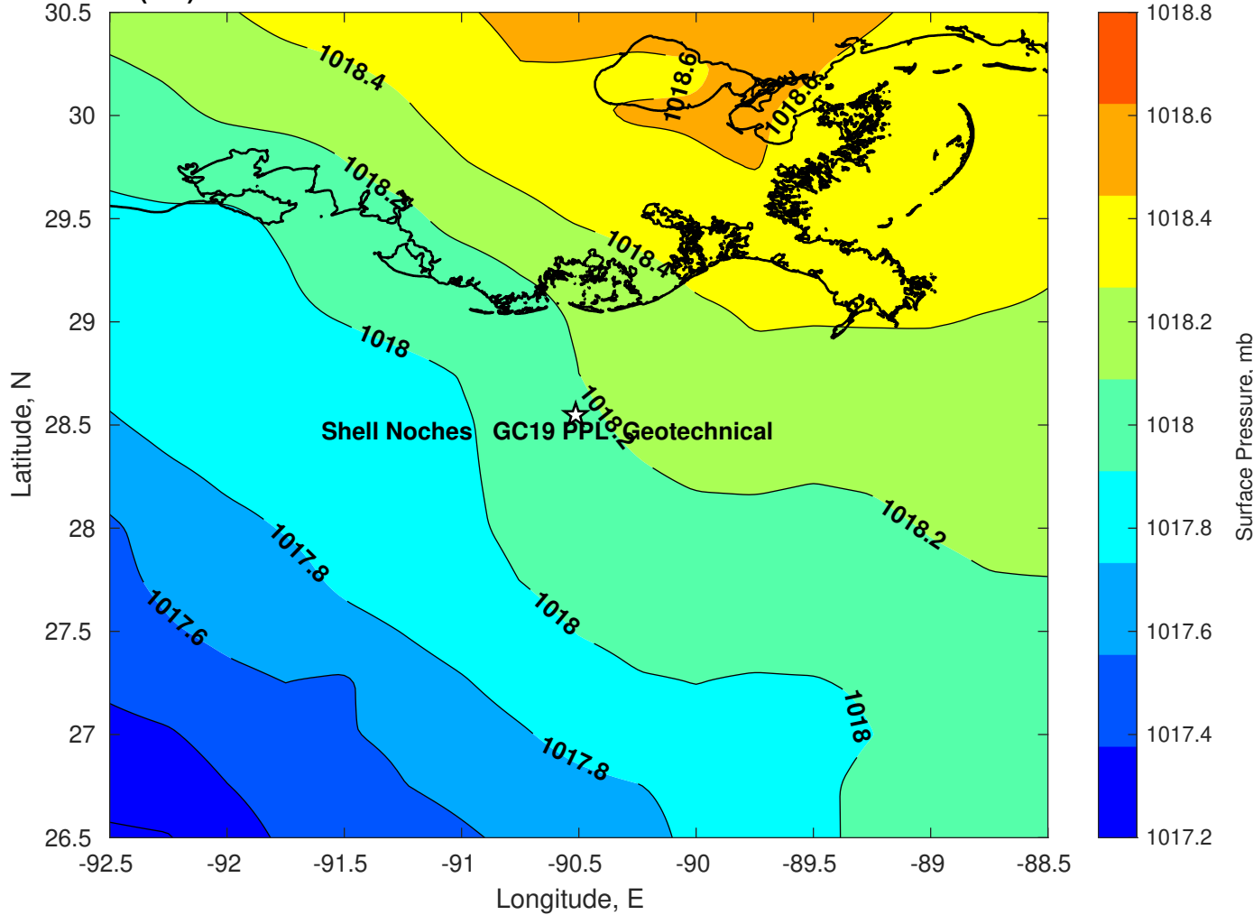
Surface Pressure (mb) for Shell Noches GC19 PPL Geotechnical at 21-Jul-2025 12:00:00
