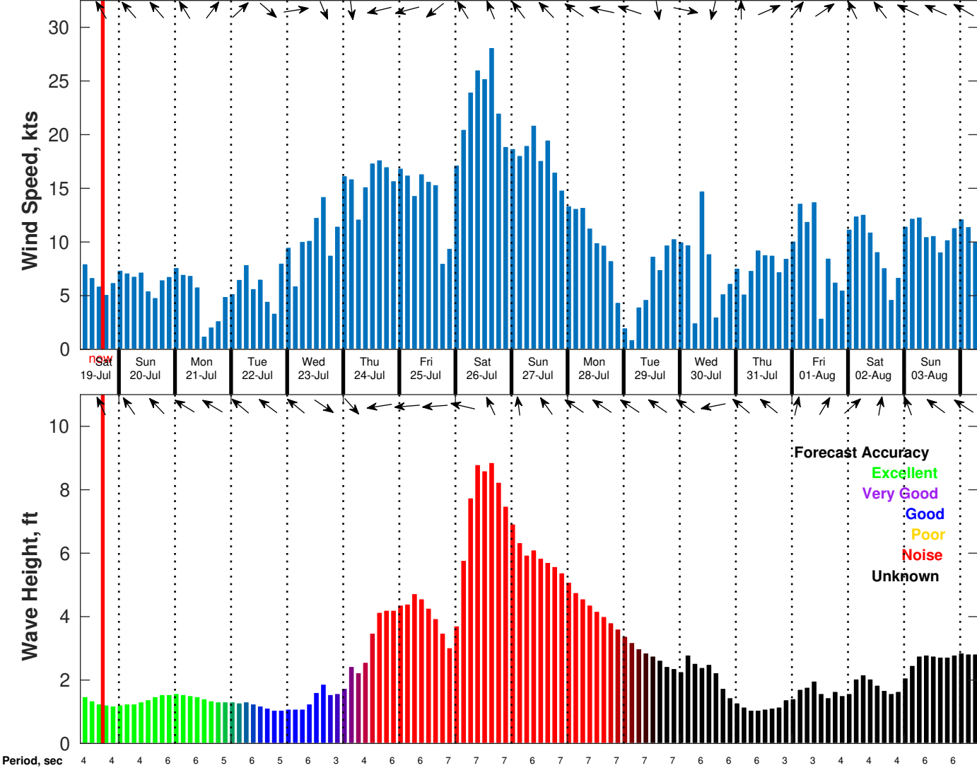
Wind & Wave Forecast for Shell Noches GC19 PPL Geotechnical from 19-Jul-2025 08:00:00 to 04-Aug-2025 08:00:00
