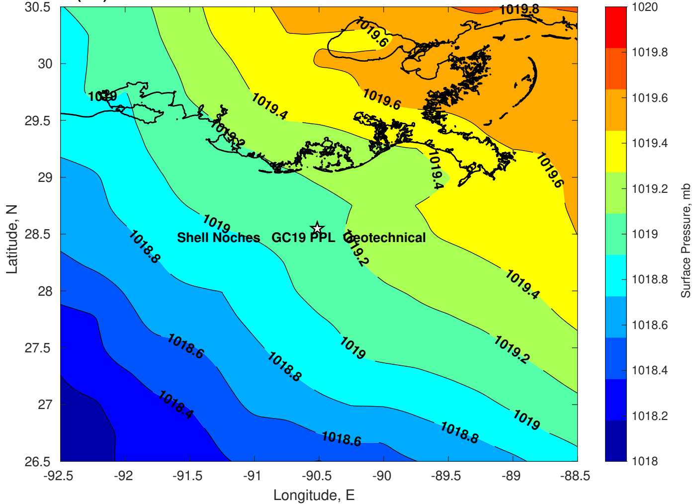
Surface Pressure (mb) for Shell Noches GC19 PPL Geotechnical at 20-Jul-2025 12:00:00
