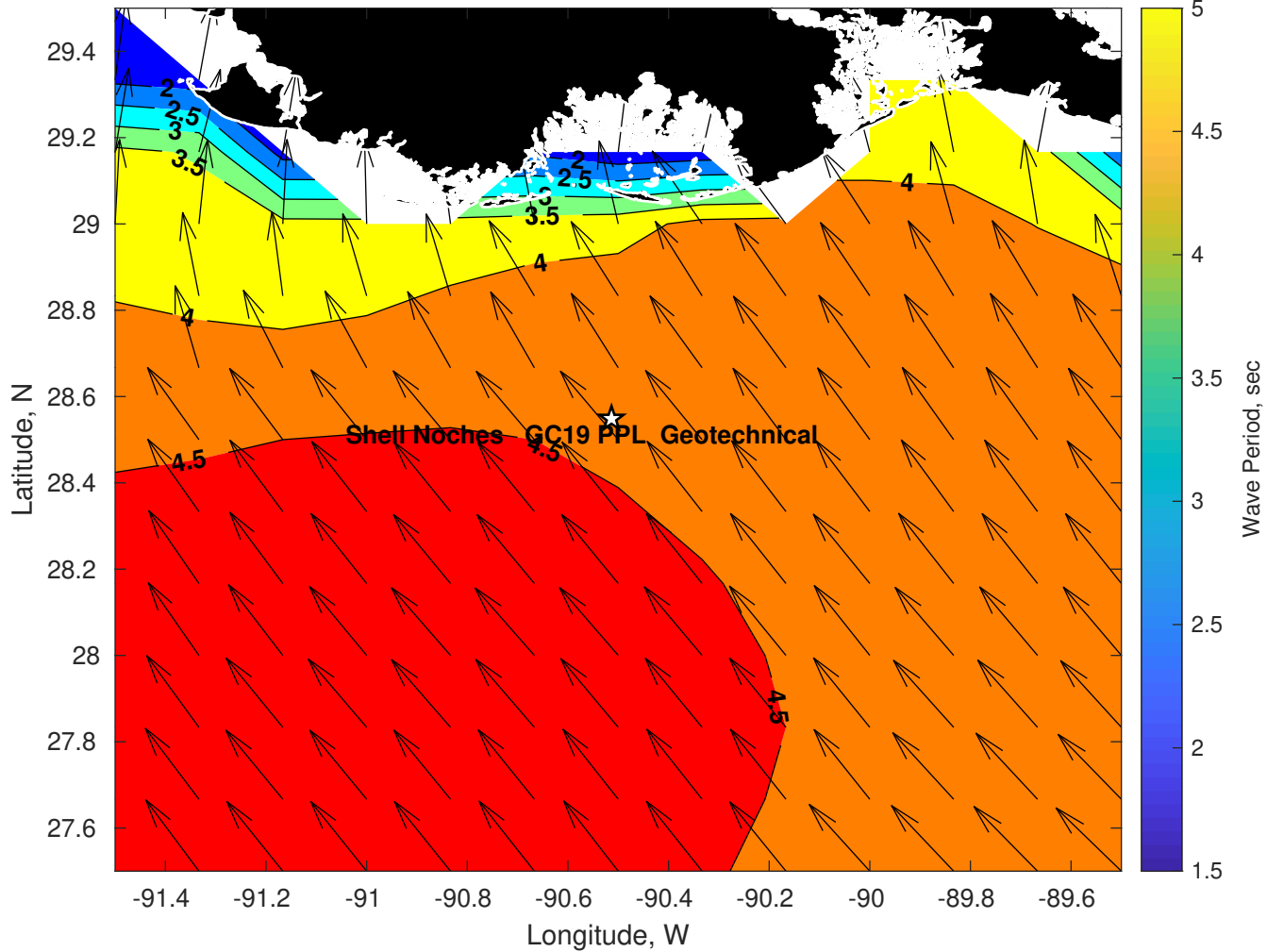
Wave Period (sec) for Shell Noches GC19 PPL Geotechnical at 19-Jul-2025 21:00:00
