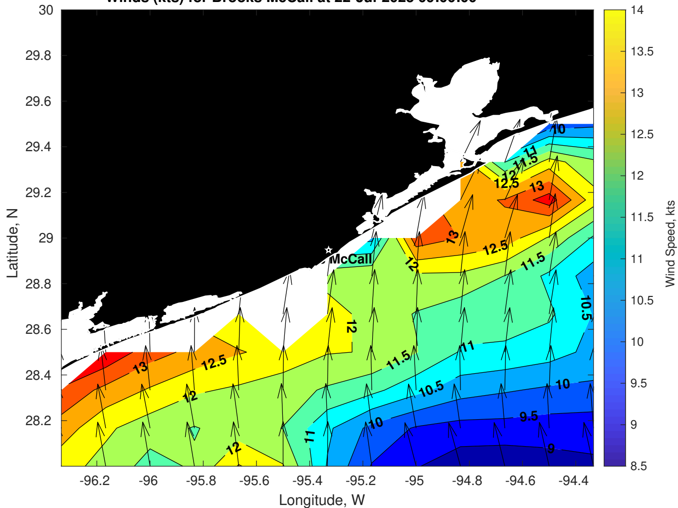
Winds (kts) for Brooks McCall at 22-Jul-2025 09:00:00
