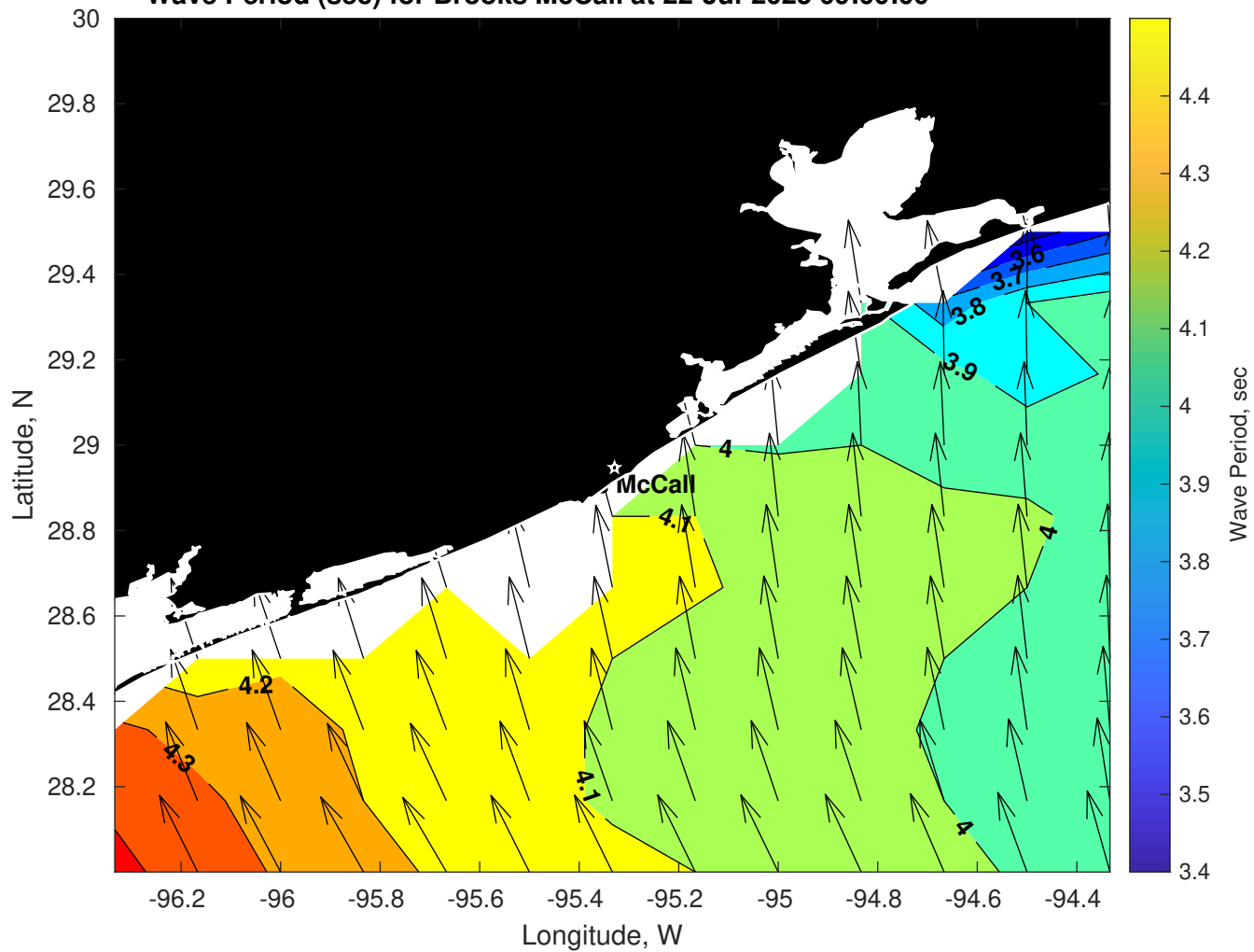
Wave Period (sec) for Brooks McCall at 22-Jul-2025 09:00:00
