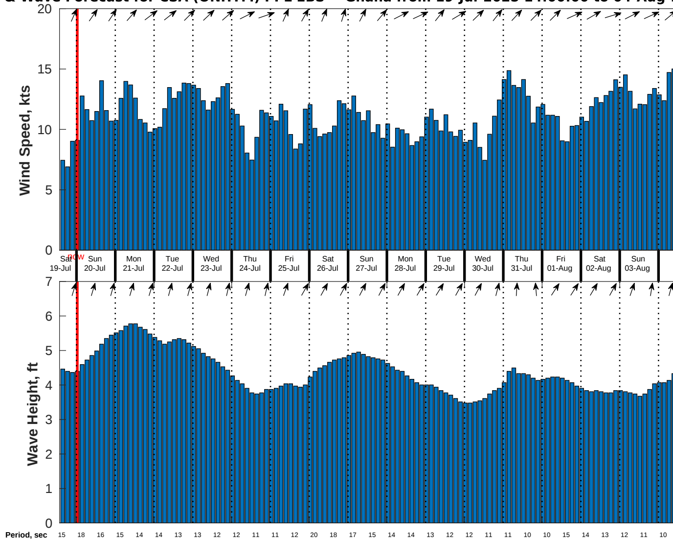
Wind & Wave Forecast for CSA (ONHYM) PPL EBS - Ghana from 19-Jul-2025 14:00:00 to 04-Aug-2025 14:00:00
