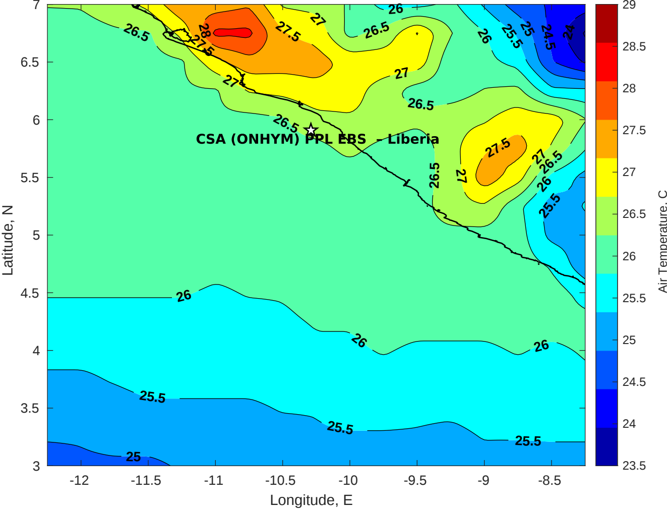
Air Temperature (C) for CSA (ONHYM) PPL EBS - Liberia at 19-Jul-2025
