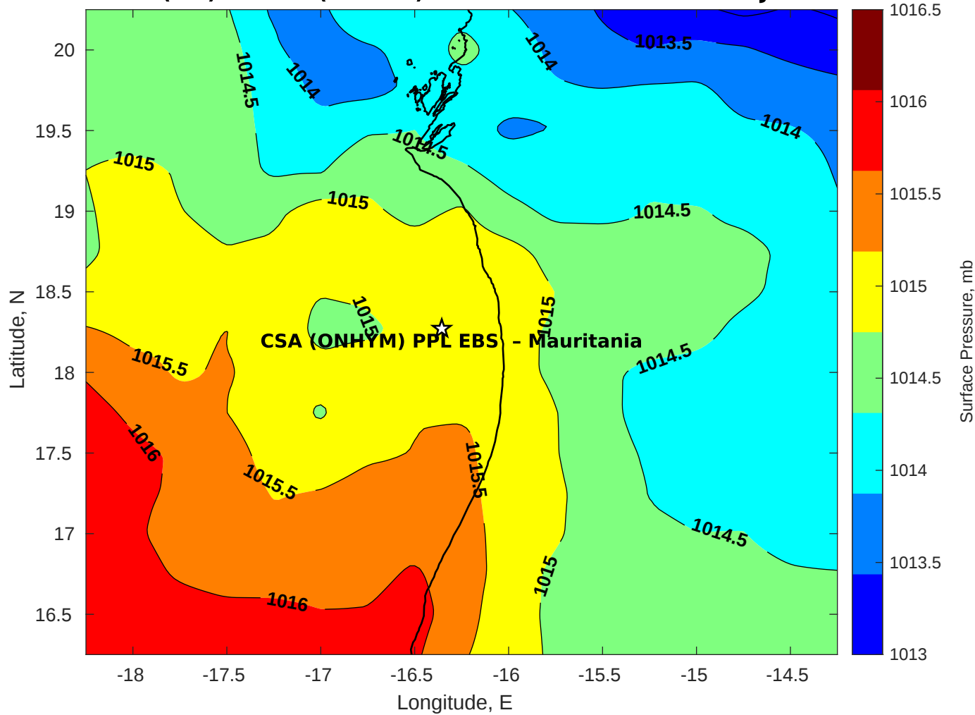
Surface Pressure (mb) for CSA (ONHYM) PPL EBS - Mauritania at 19-Jul-2025 12:00:00
