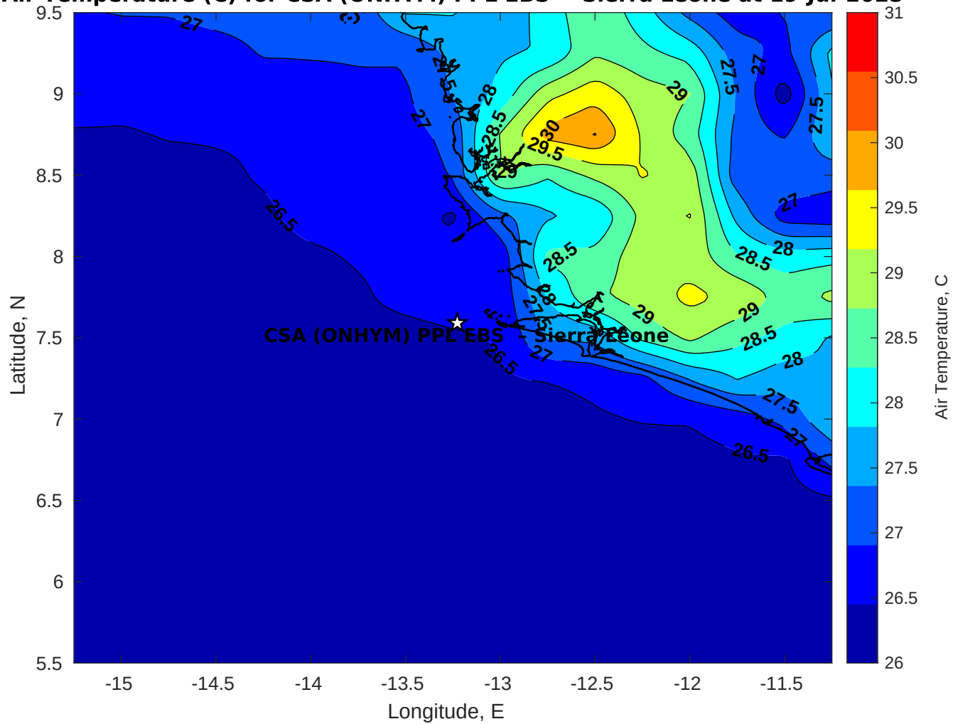
Air Temperature (C) for CSA (ONHYM) PPL EBS - Sierra Leone at 19-Jul-2025
