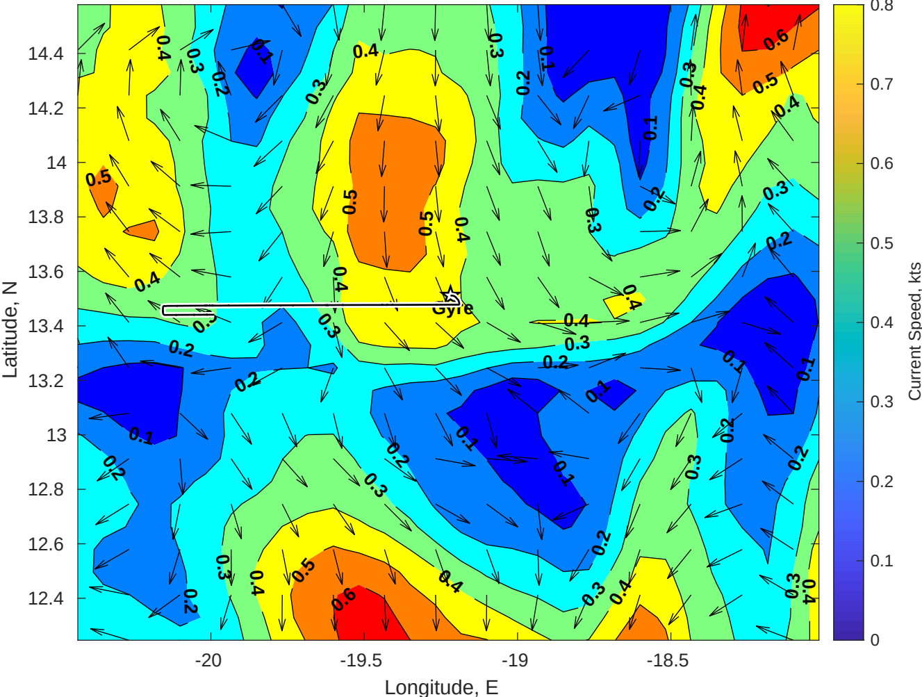
Surface Currents for Gyre at 21-Jul-2025 00:00:00
