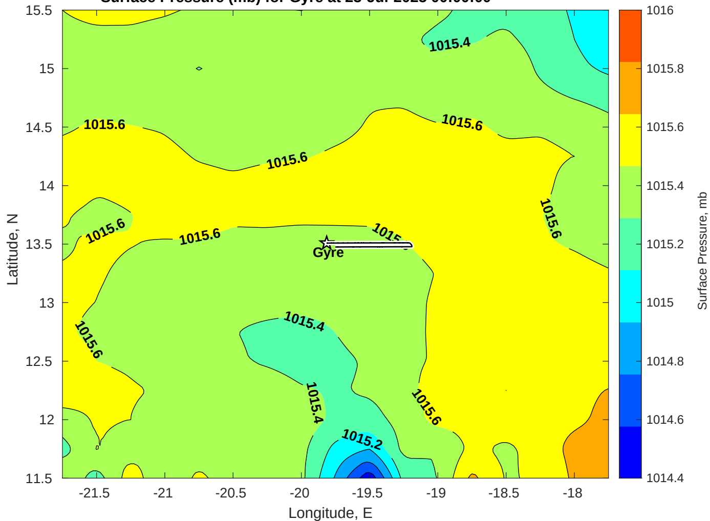
Surface Pressure (mb) for Gyre at 23-Jul-2025 00:00:00
