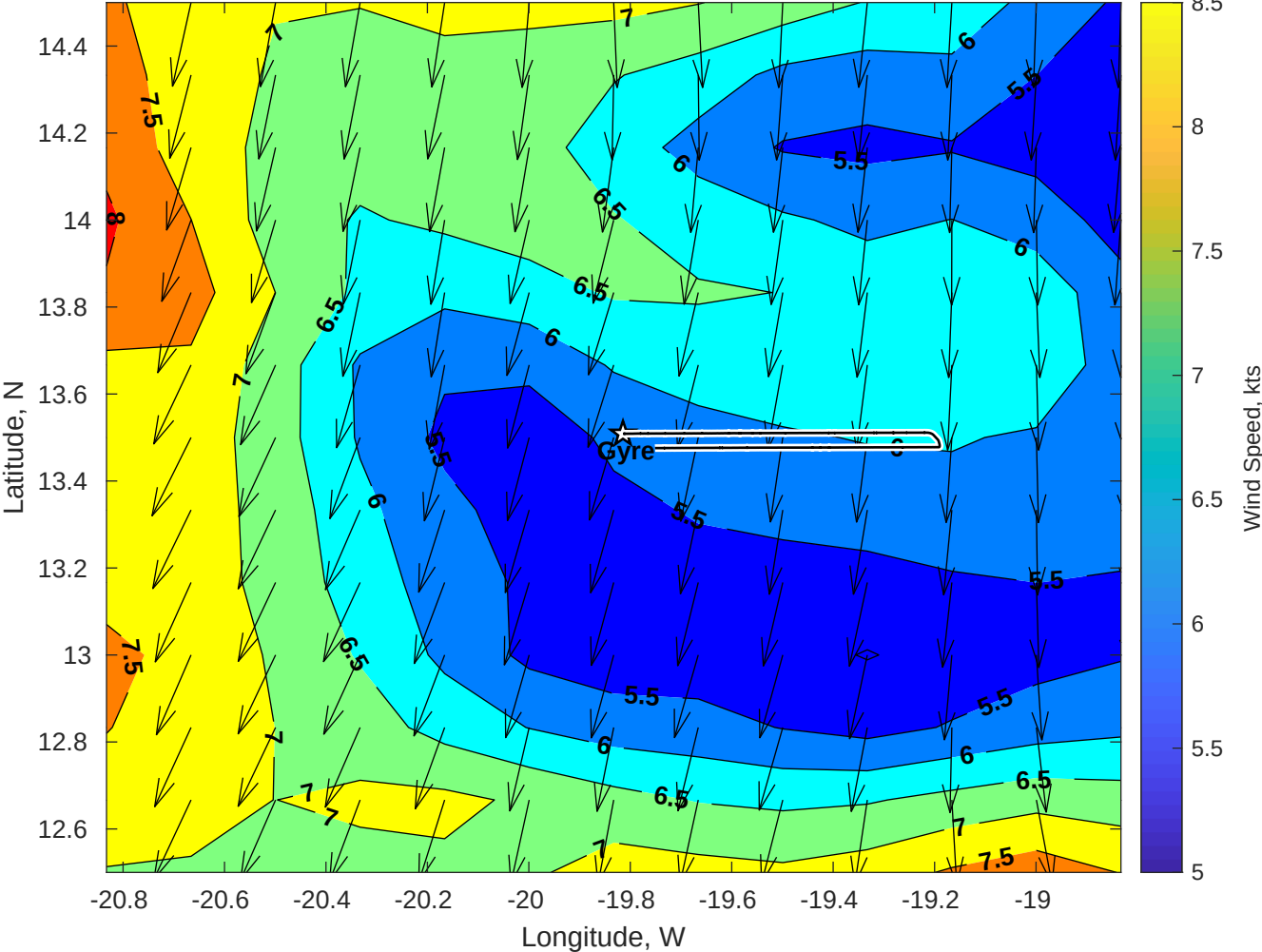
Winds (kts) for Gyre at 22-Jul-2025 09:00:00
