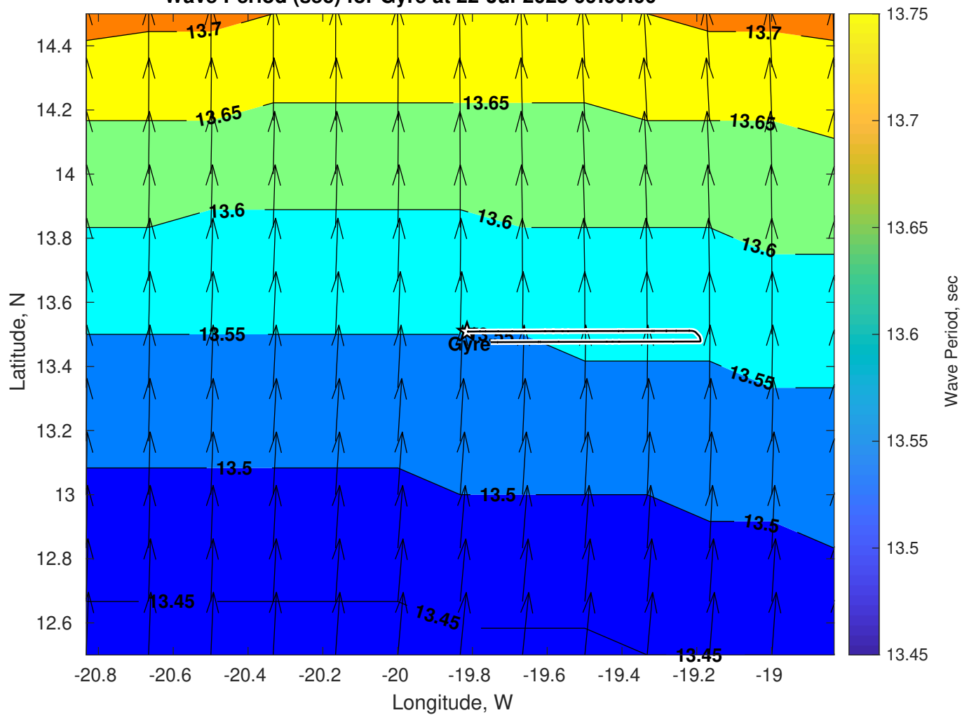
Wave Period (sec) for Gyre at 22-Jul-2025 09:00:00
