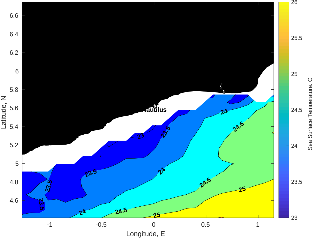
SST for Nautilus at 19-Jul-2025 00:00:00
