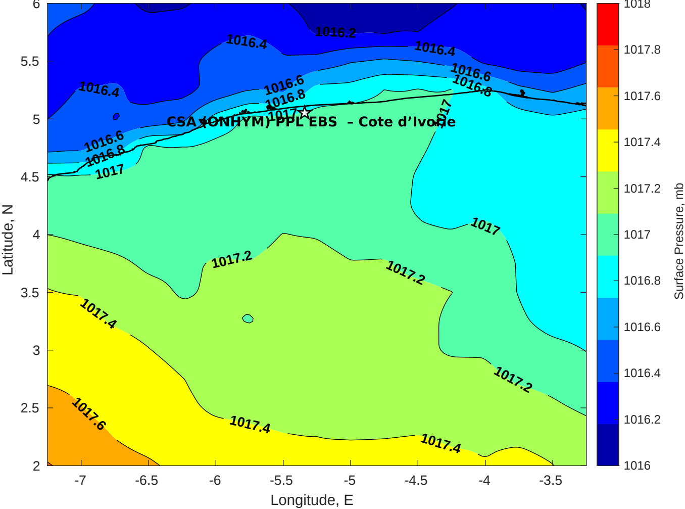
Surface Pressure (mb) for CSA (ONHYM) PPL EBS - Cote d'Ivoire at 19-Jul-2025 12:00:00
