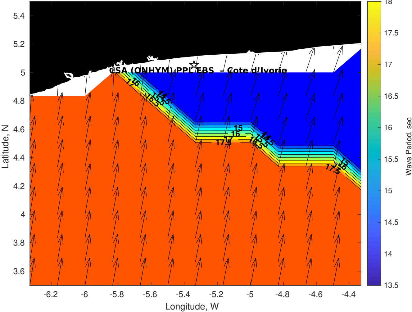
Wave Period (sec) for CSA (ONHYM) PPL EBS - Cote d'Ivoire at 19-Jul-2025 21:00:00
